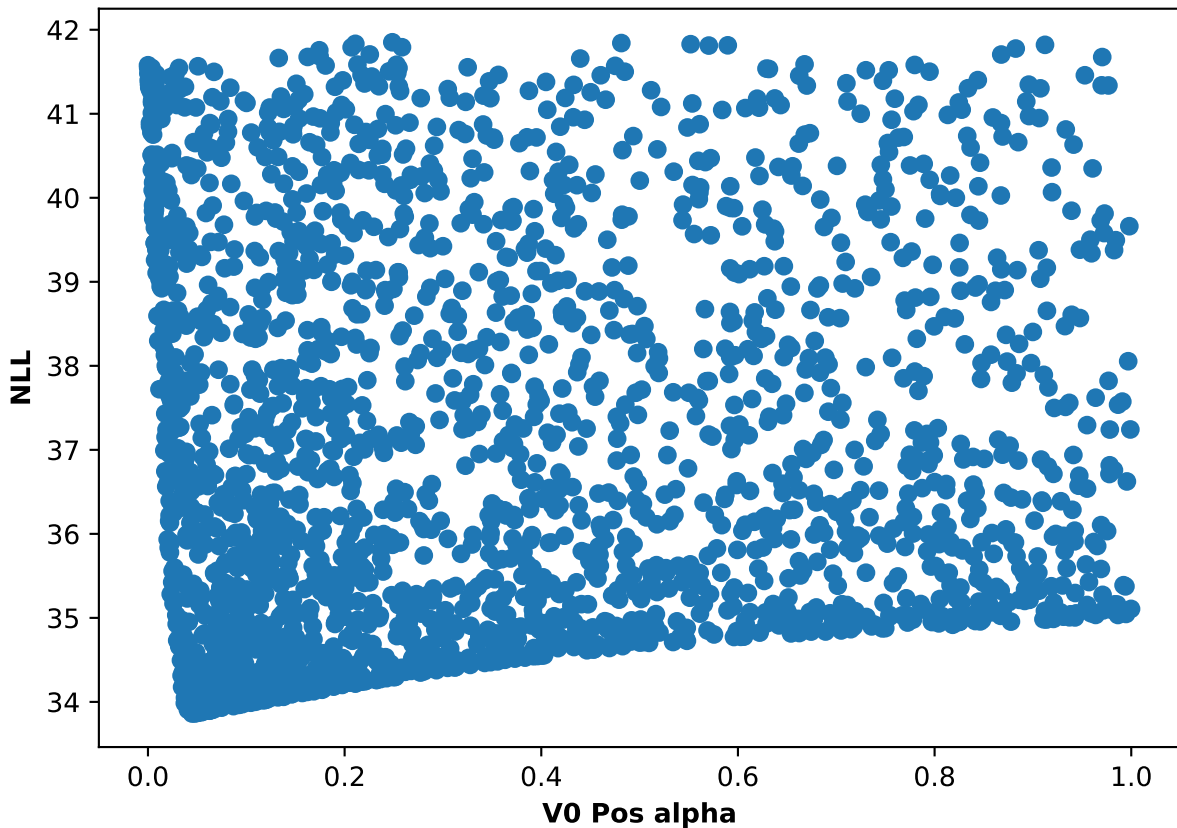
Participant 28, run 5: NLL and V0 Pos alpha scatter plot
