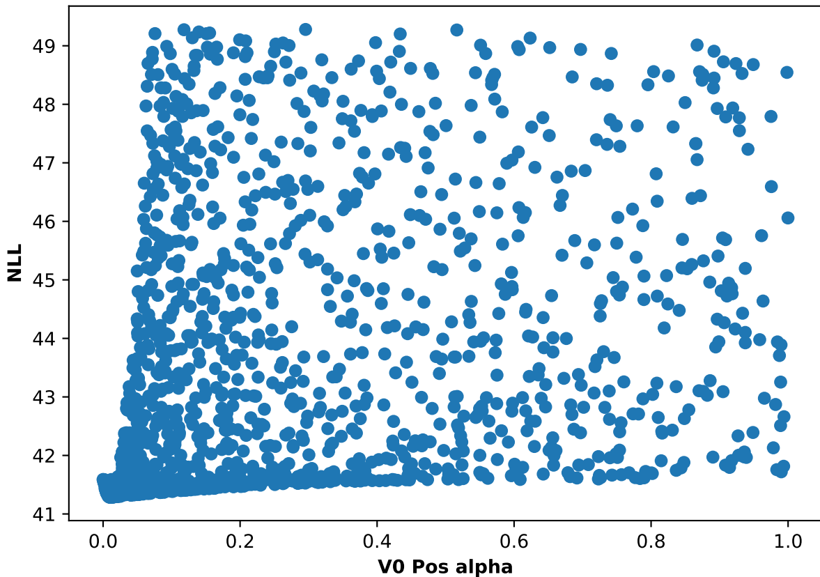
Participant 29, run 1: NLL and V0 Pos alpha scatter plot
