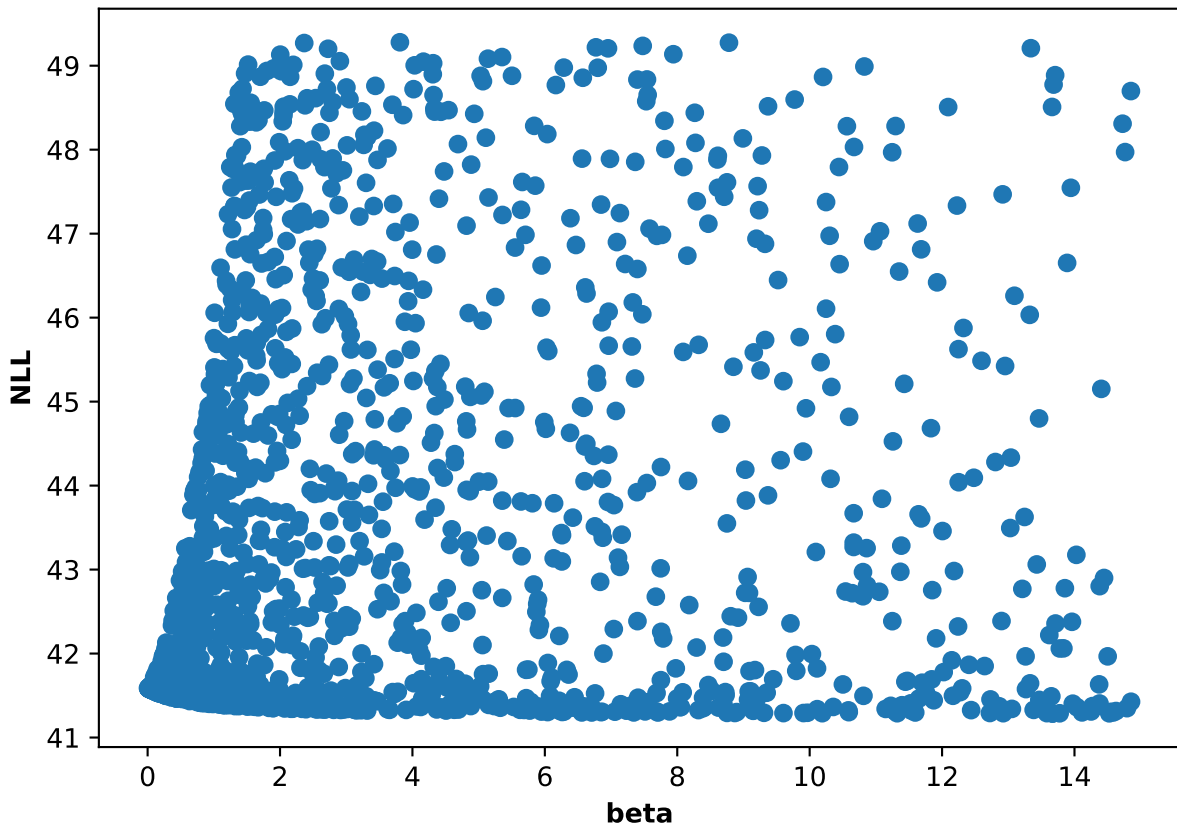
Participant 29, run 1: NLL and beta scatter plot
