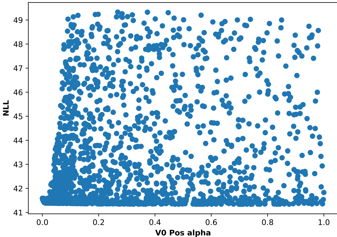
Participant 29, run 2: NLL and V0 Pos alpha scatter plot
