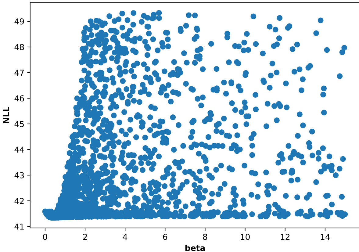
Participant 29, run 2: NLL and beta scatter plot
