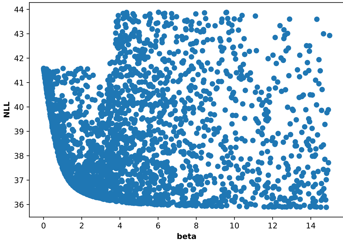
Participant 29, run 4: NLL and beta scatter plot
