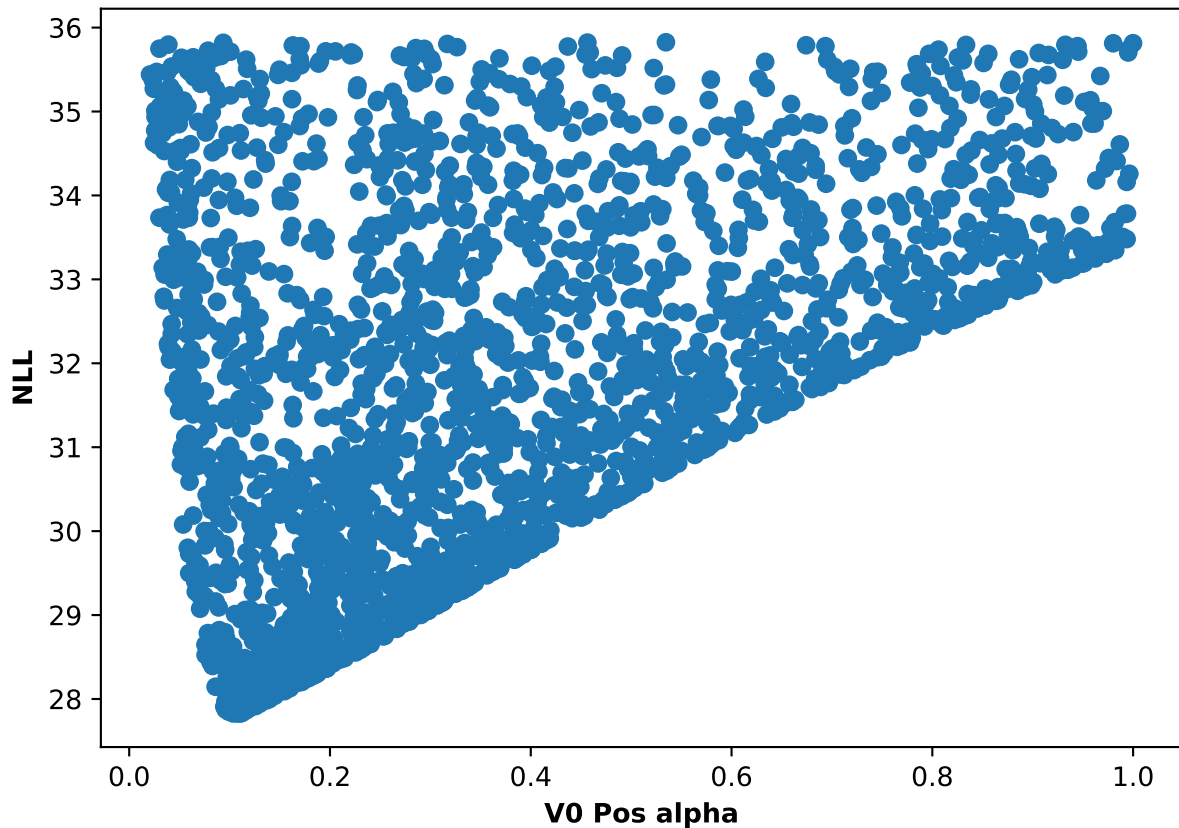
Participant 29, run 5: NLL and V0 Pos alpha scatter plot
