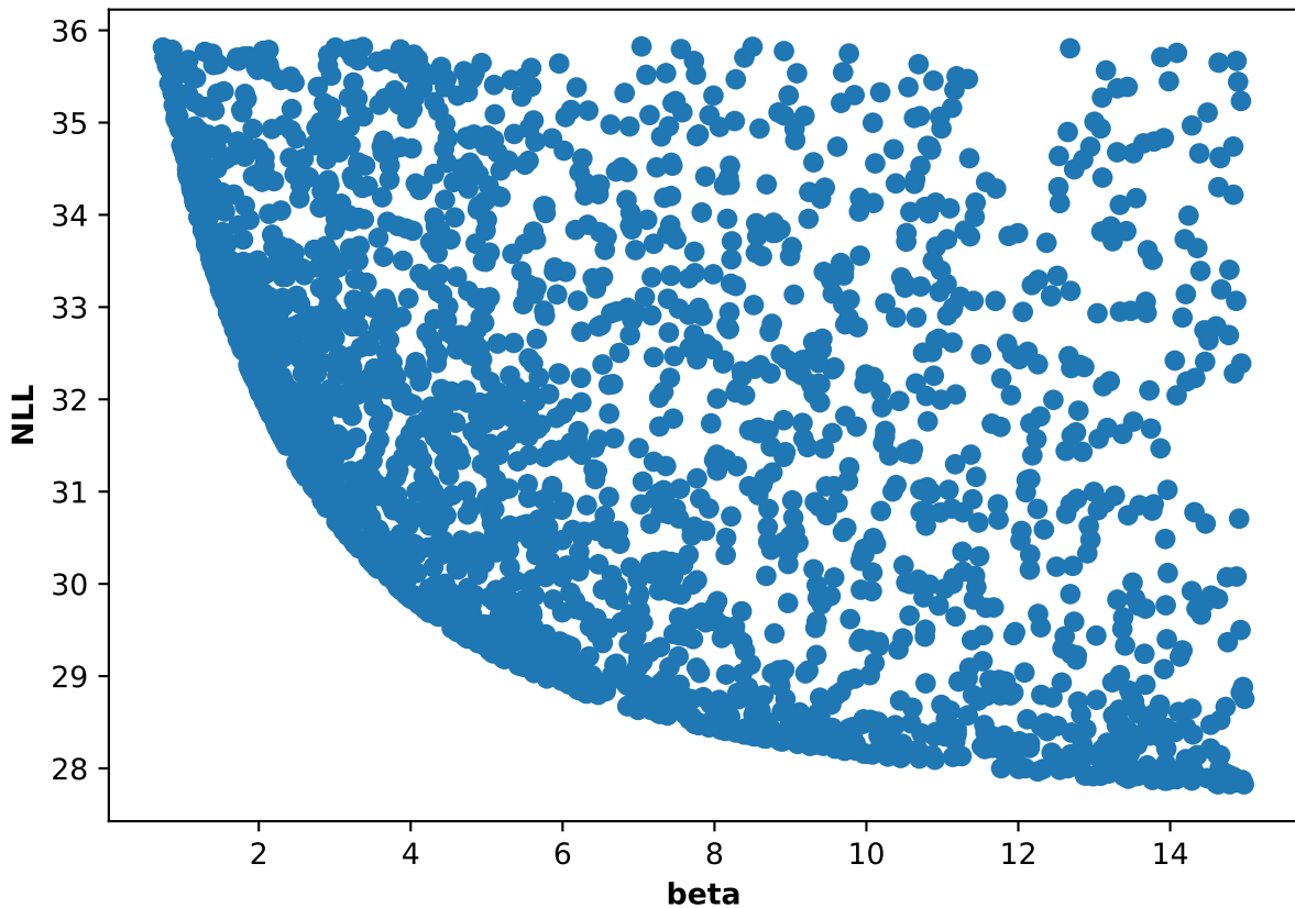
Participant 29, run 5: NLL and beta scatter plot
