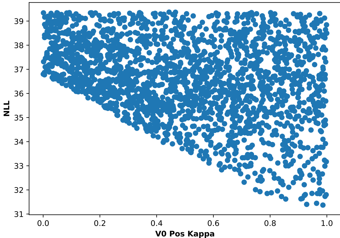
Participant 30, run 4: NLL and V0 Pos Kappa scatter plot
