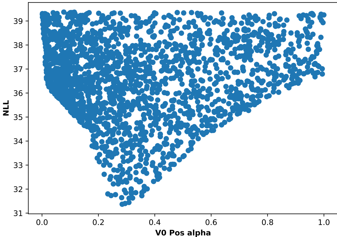
Participant 30, run 4: NLL and V0 Pos alpha scatter plot
