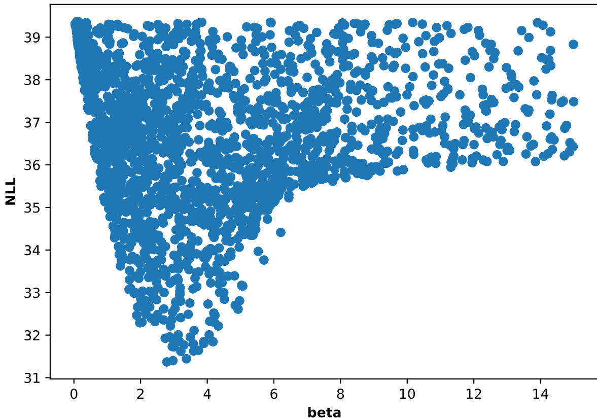
Participant 30, run 4: NLL and beta scatter plot
