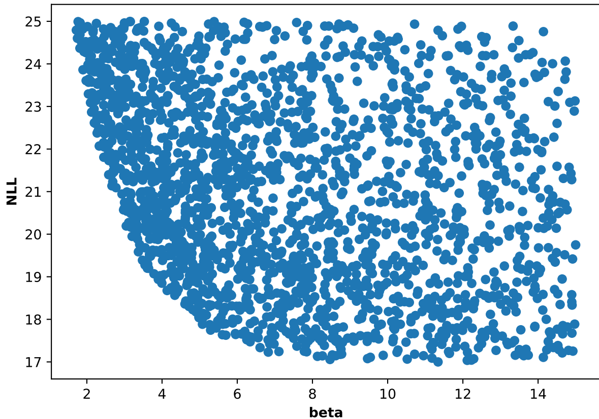
Participant 30, run 5: NLL and beta scatter plot
