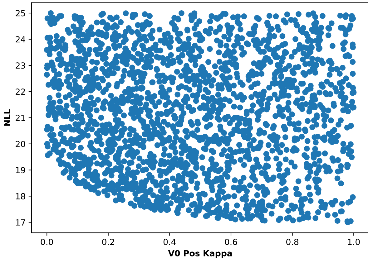
Participant 30, run 5: NLL and V0 Pos Kappa scatter plot
