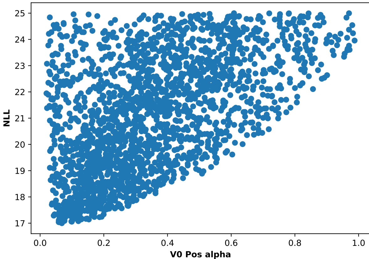
Participant 30, run 5: NLL and V0 Pos alpha scatter plot
