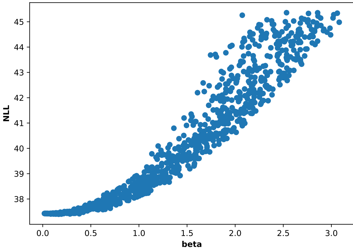
Participant 33, run 1: NLL and beta scatter plot
