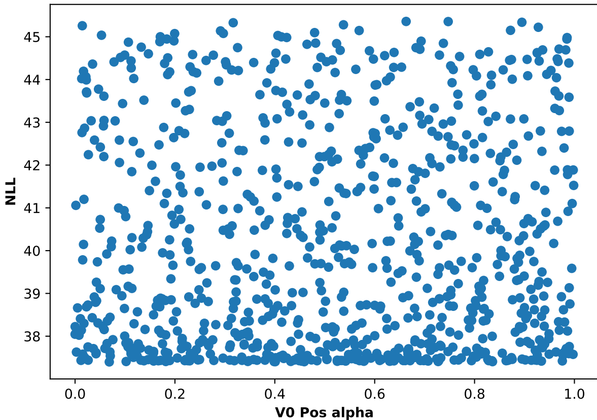
Participant 33, run 1: NLL and V0 Pos alpha scatter plot
