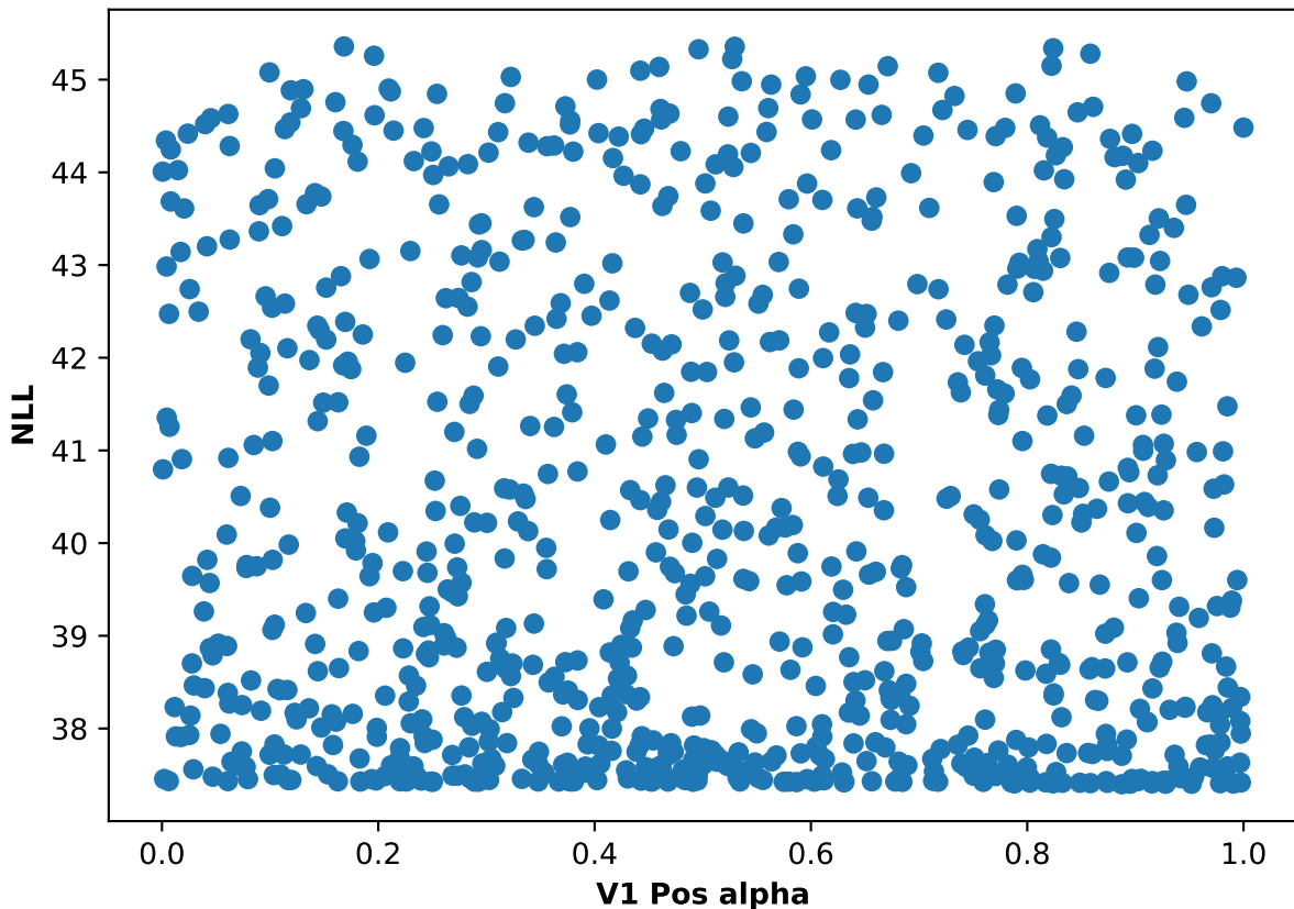
Participant 33, run 1: NLL and V1 Pos alpha scatter plot
