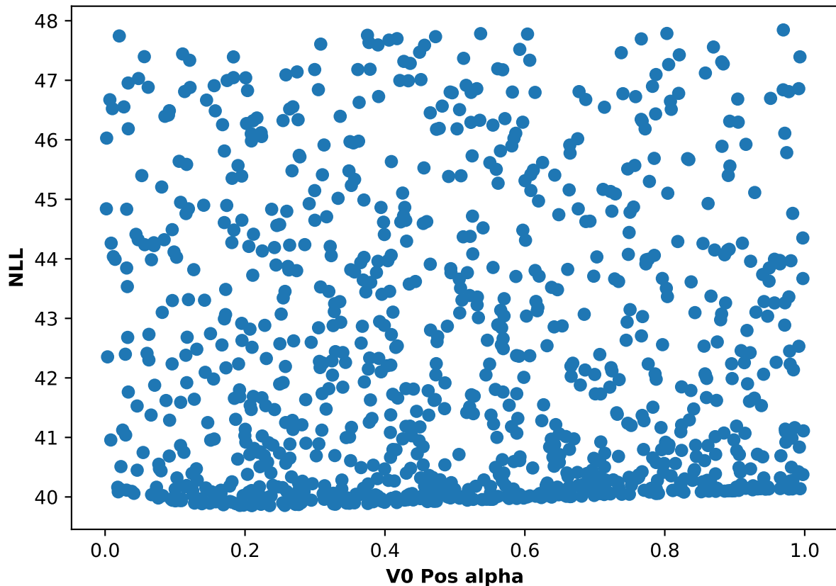
Participant 34, run 1: NLL and V0 Pos alpha scatter plot
