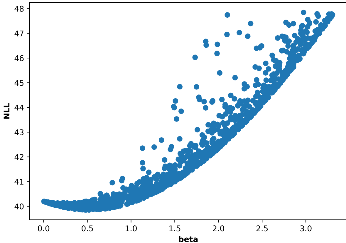
Participant 34, run 1: NLL and beta scatter plot
