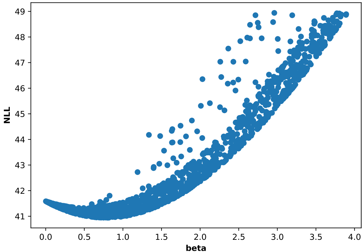
Participant 34, run 2: NLL and beta scatter plot
