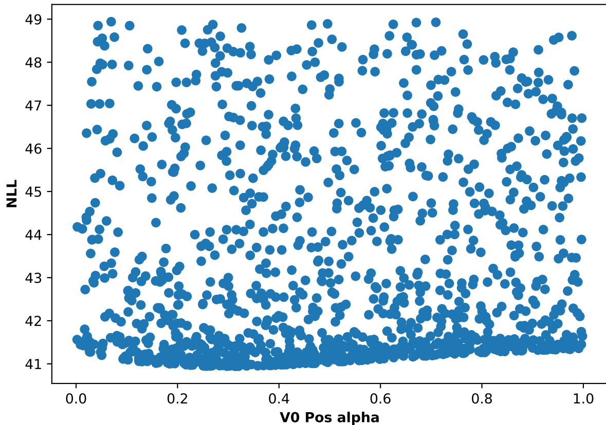
Participant 34, run 2: NLL and V0 Pos alpha scatter plot
