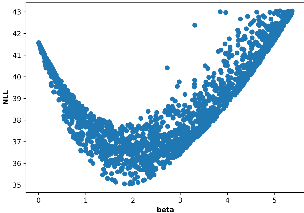
Participant 34, run 4: NLL and beta scatter plot
