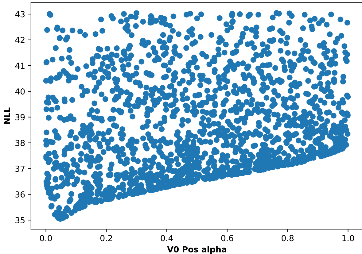
Participant 34, run 4: NLL and V0 Pos alpha scatter plot
