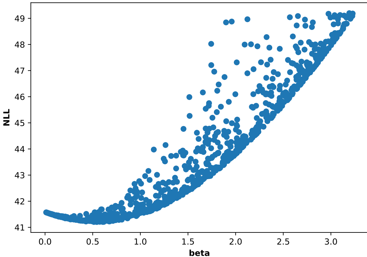
Participant 35, run 2: NLL and beta scatter plot
