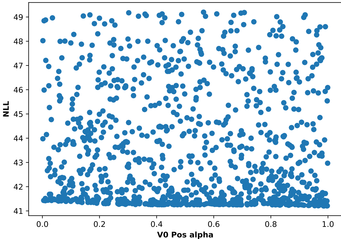
Participant 35, run 2: NLL and V0 Pos alpha scatter plot
