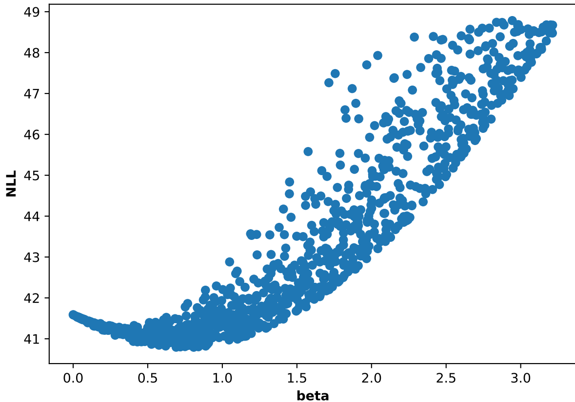
Participant 35, run 3: NLL and beta scatter plot
