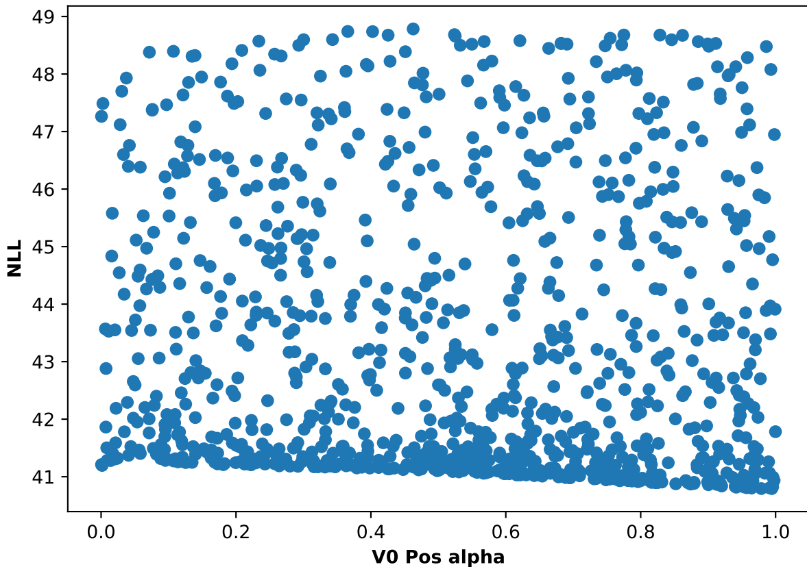
Participant 35, run 3: NLL and V0 Pos alpha scatter plot
