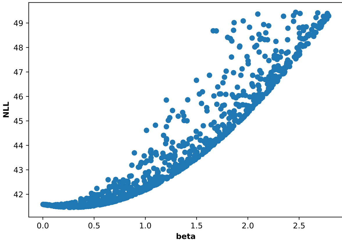
Participant 35, run 5: NLL and beta scatter plot
