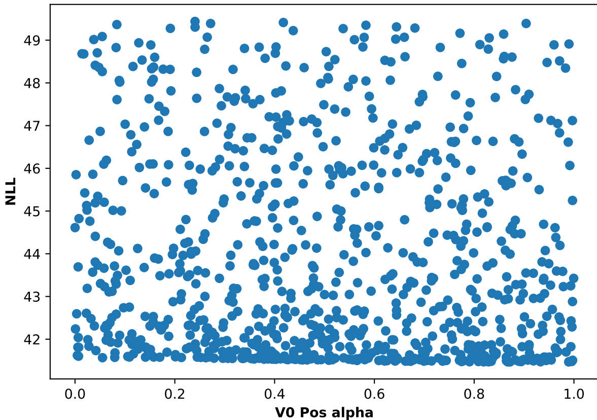
Participant 35, run 5: NLL and V0 Pos alpha scatter plot
