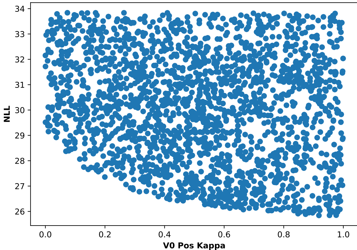
Participant 36, run 2: NLL and V0 Pos Kappa scatter plot
