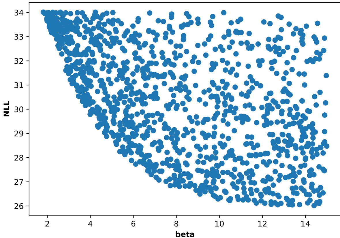
Participant 36, run 3: NLL and beta scatter plot
