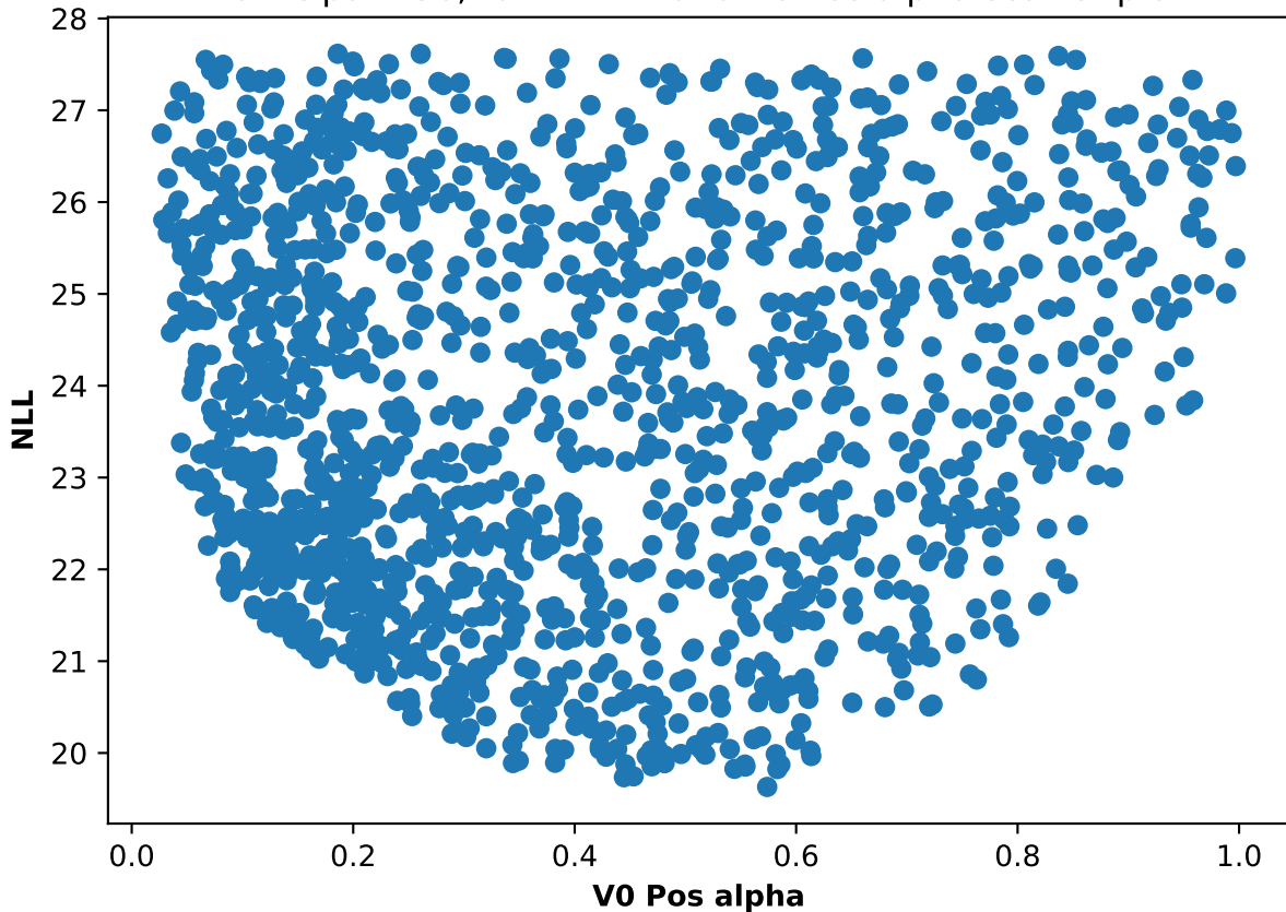
Participant 36, run 4: NLL and V0 Pos alpha scatter plot
