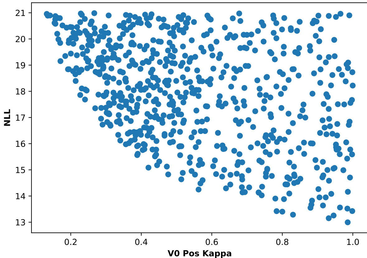
Participant 36, run 5: NLL and V0 Pos Kappa scatter plot
