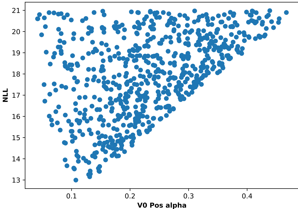
Participant 36, run 5: NLL and V0 Pos alpha scatter plot
