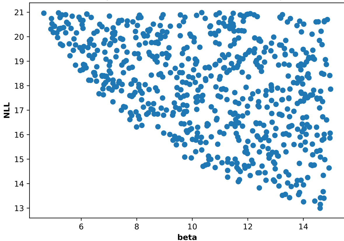
Participant 36, run 5: NLL and beta scatter plot
