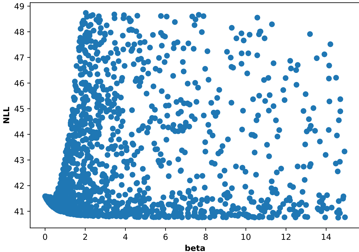
Participant 37, run 5: NLL and beta scatter plot
