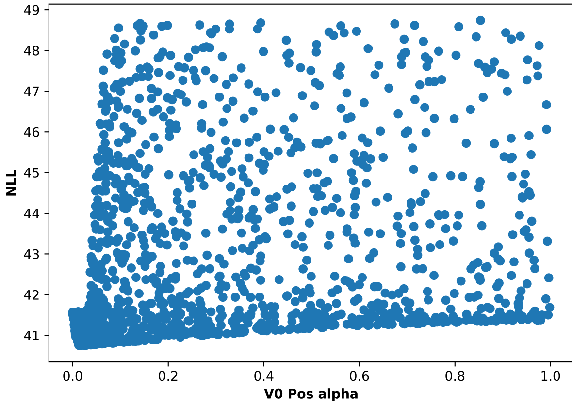
Participant 37, run 5: NLL and V0 Pos alpha scatter plot
