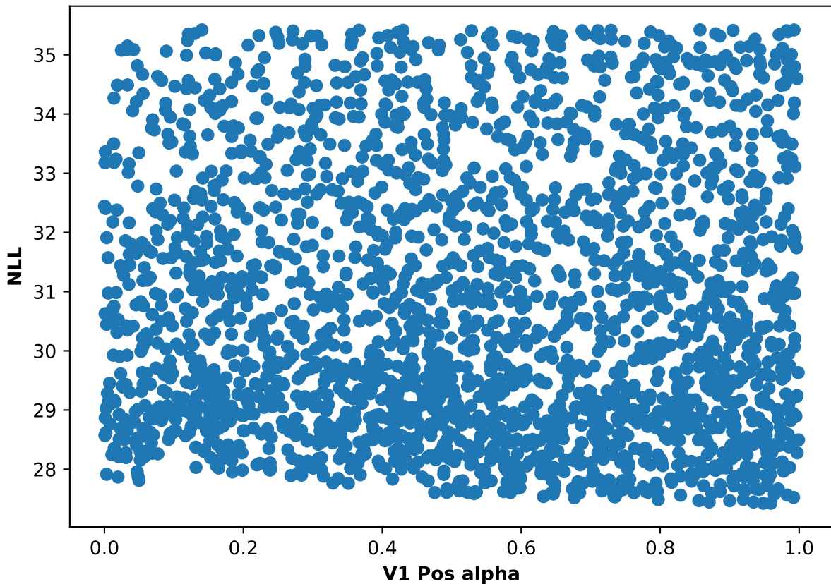
Participant 38, run 5: NLL and V1 Pos alpha scatter plot
