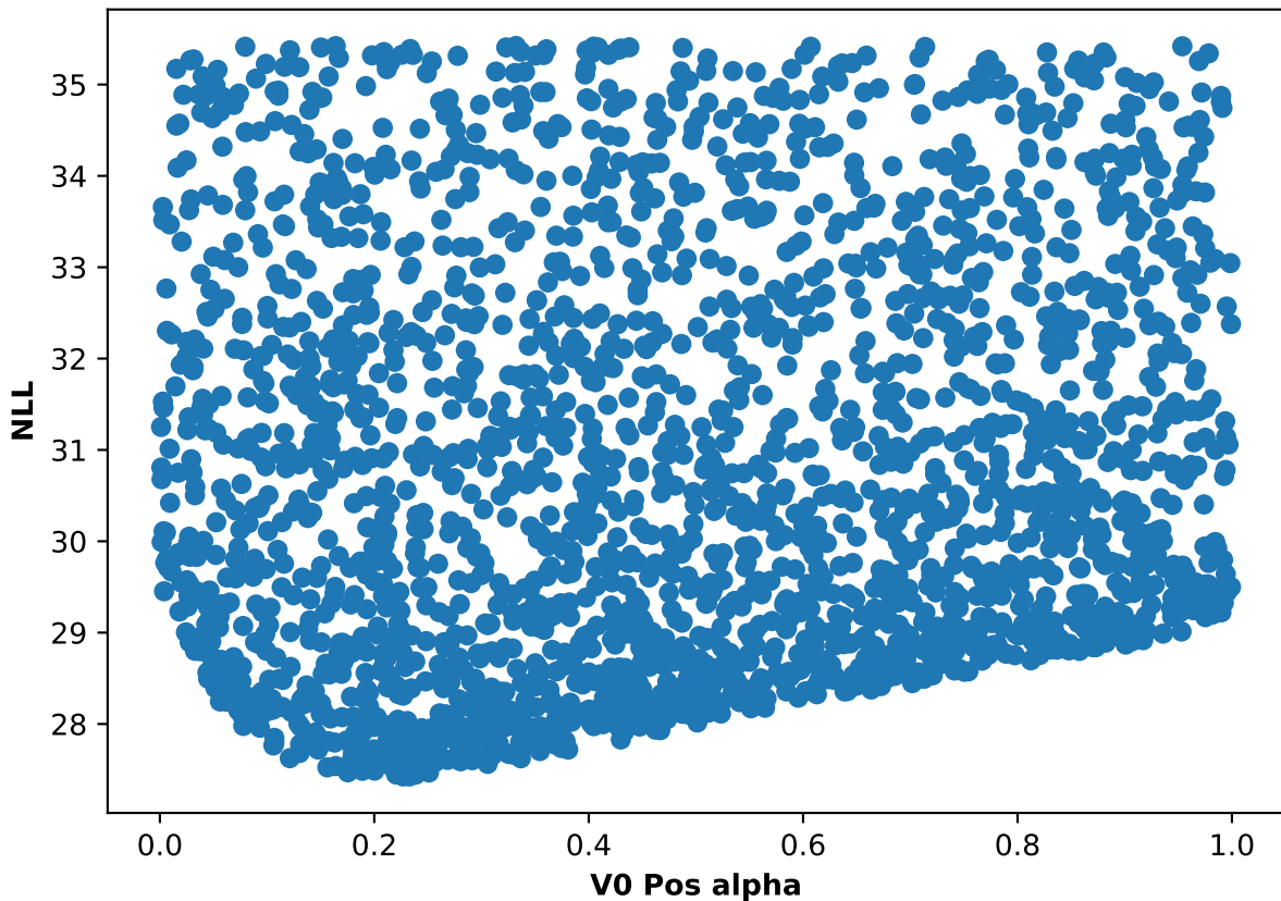
Participant 38, run 5: NLL and V0 Pos alpha scatter plot
