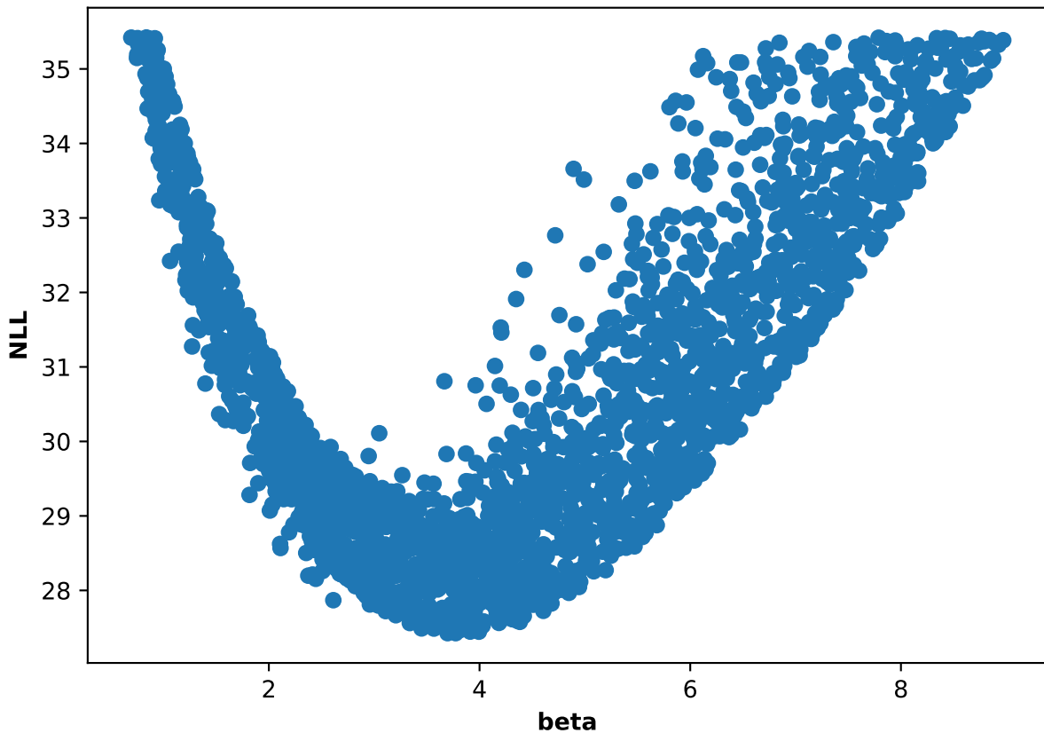
Participant 38, run 5: NLL and beta scatter plot
