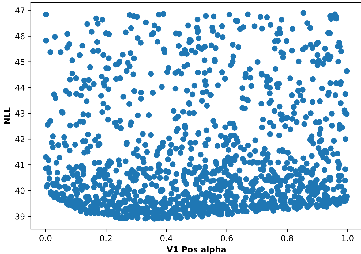
Participant 39, run 1: NLL and V1 Pos alpha scatter plot
