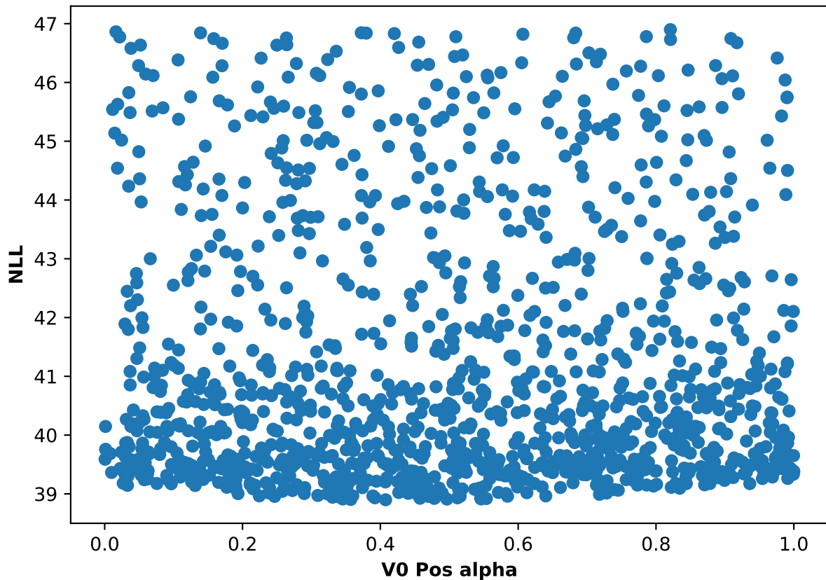
Participant 39, run 1: NLL and V0 Pos alpha scatter plot
