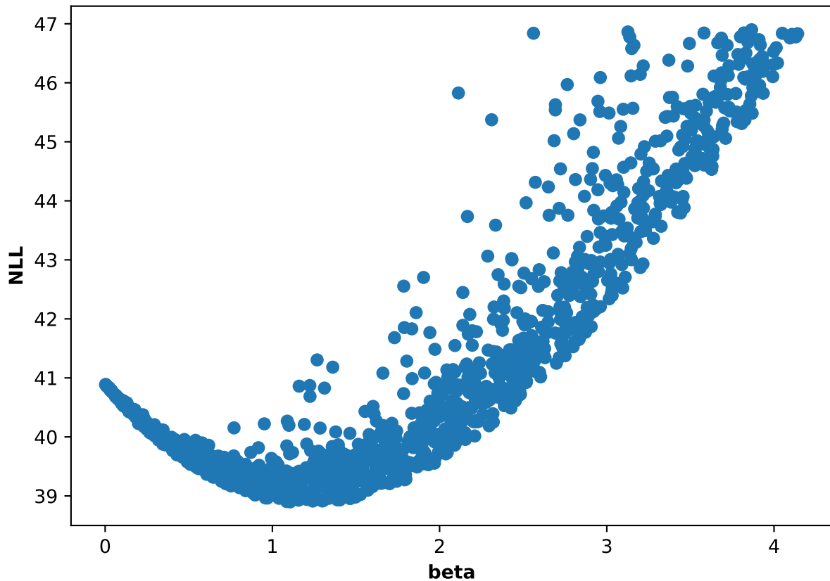
Participant 39, run 1: NLL and beta scatter plot
