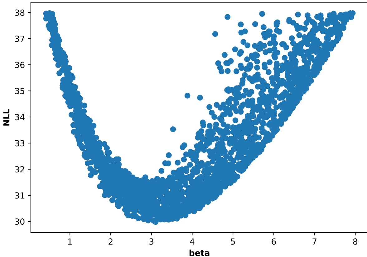
Participant 39, run 2: NLL and beta scatter plot
