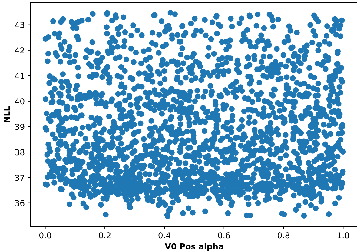
Participant 39, run 4: NLL and V0 Pos alpha scatter plot
