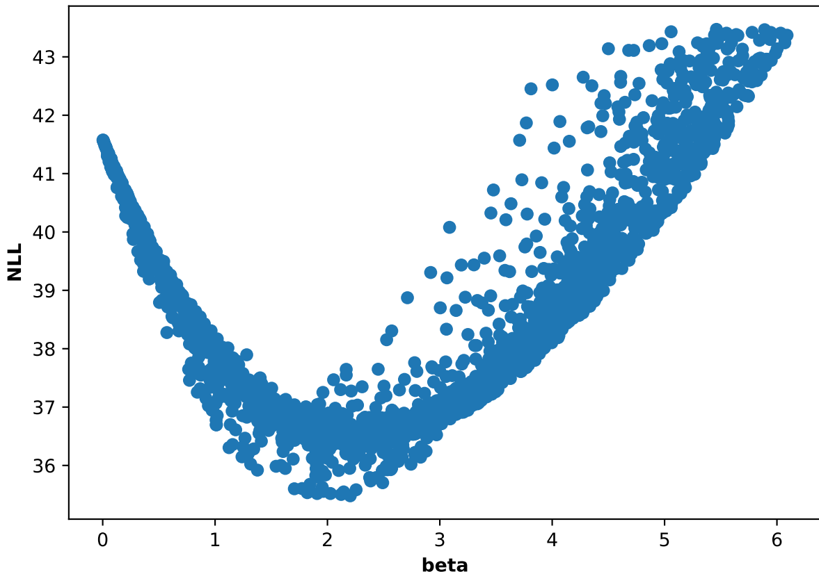
Participant 39, run 4: NLL and beta scatter plot
