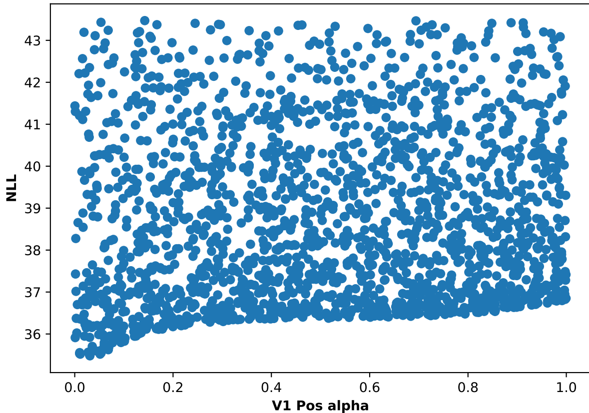
Participant 39, run 4: NLL and V1 Pos alpha scatter plot
