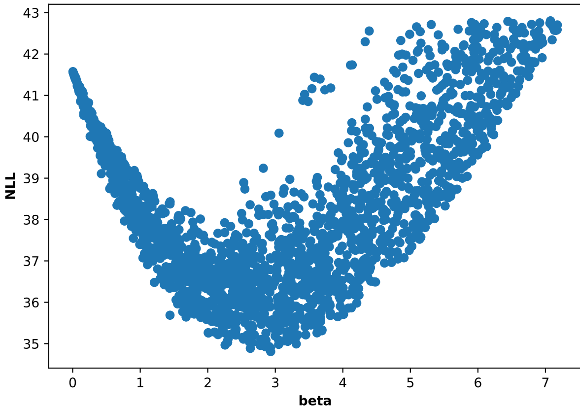
Participant 40, run 4: NLL and beta scatter plot
