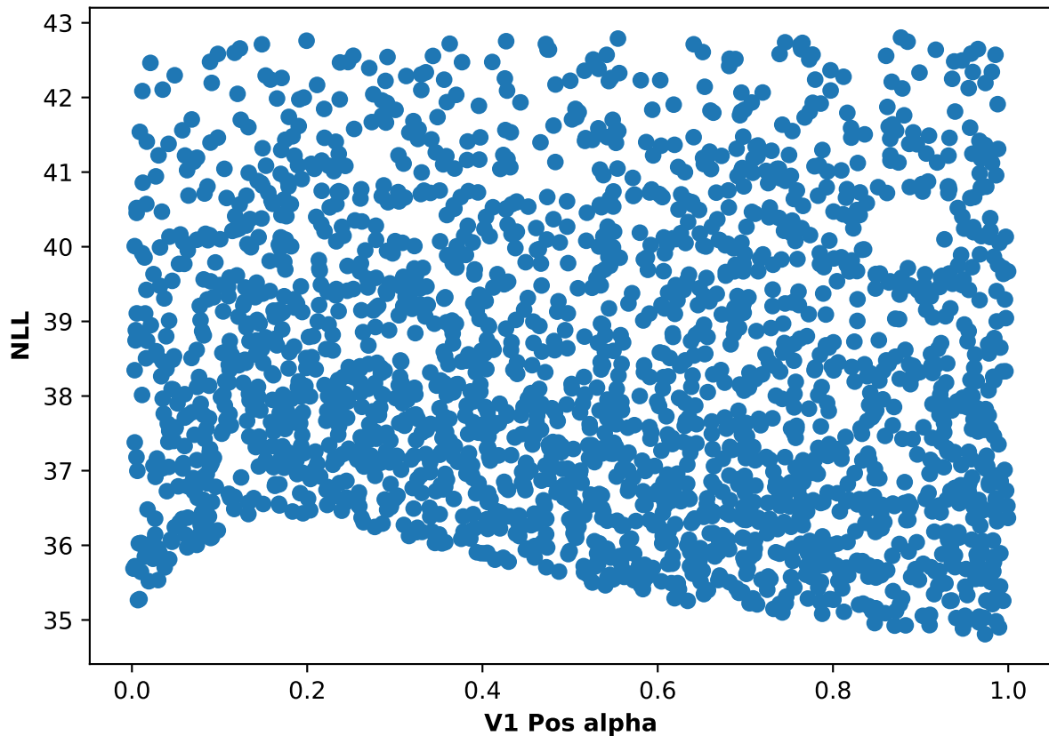
Participant 40, run 4: NLL and V1 Pos alpha scatter plot
