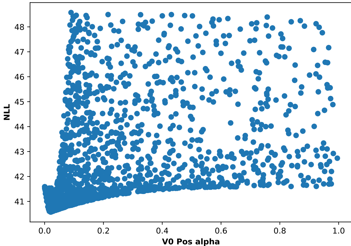
Participant 41, run 1: NLL and V0 Pos alpha scatter plot
