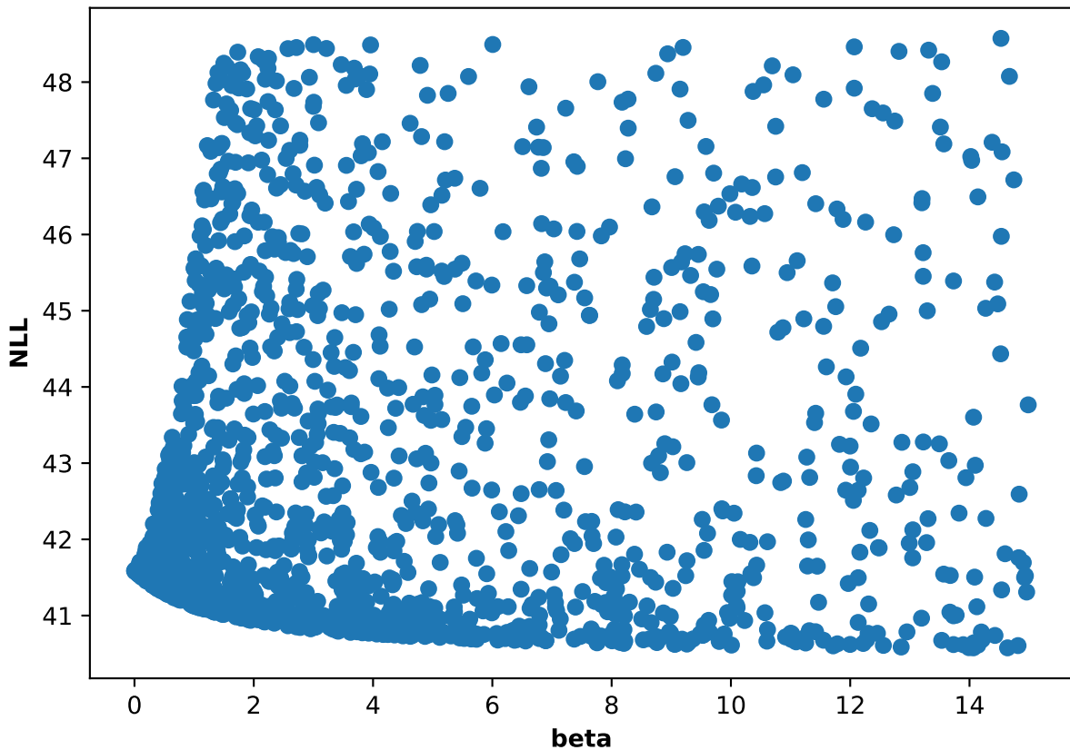
Participant 41, run 1: NLL and beta scatter plot
