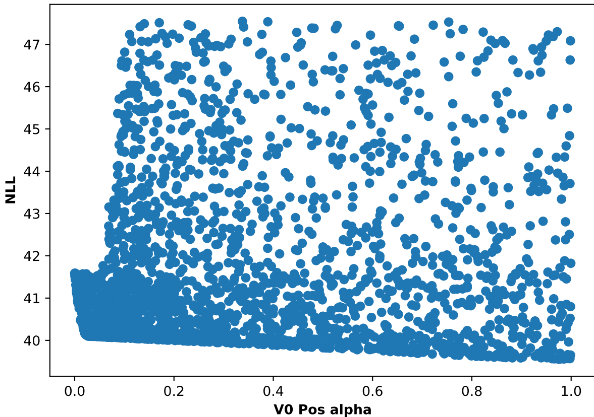
Participant 41, run 2: NLL and V0 Pos alpha scatter plot
