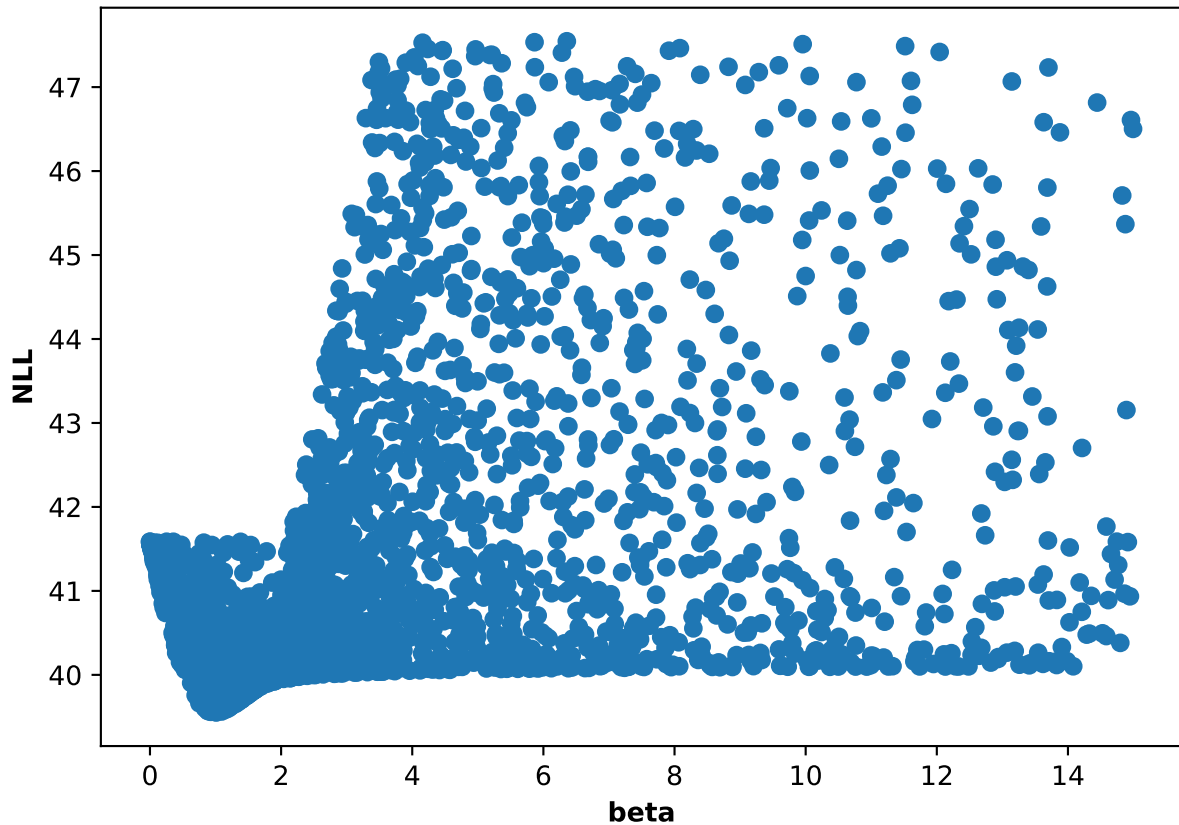
Participant 41, run 2: NLL and beta scatter plot
