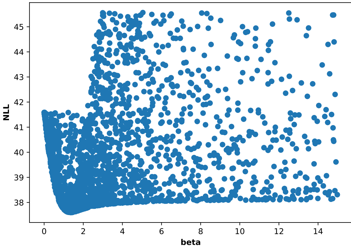
Participant 41, run 4: NLL and beta scatter plot
