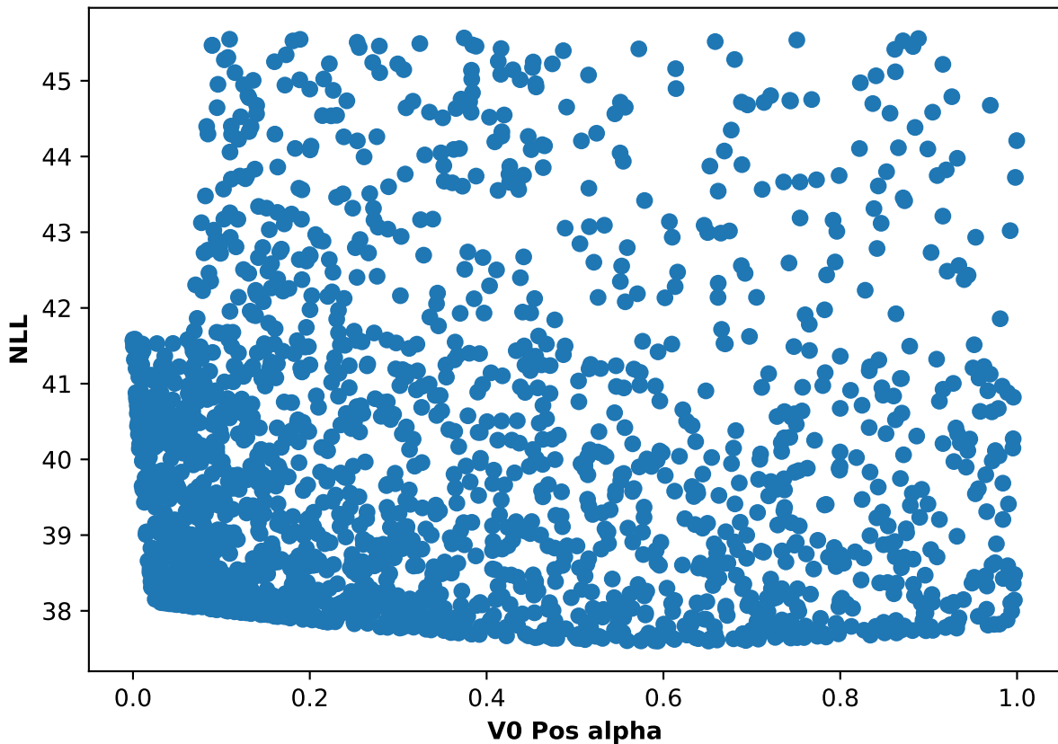
Participant 41, run 4: NLL and V0 Pos alpha scatter plot
