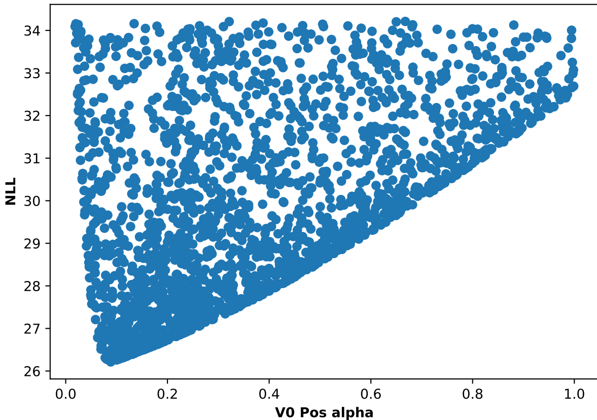
Participant 41, run 5: NLL and V0 Pos alpha scatter plot
