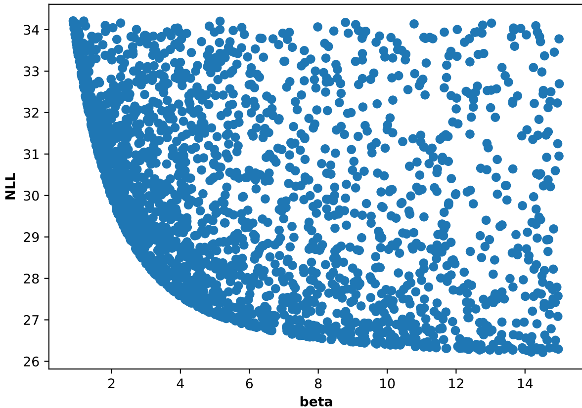
Participant 41, run 5: NLL and beta scatter plot
