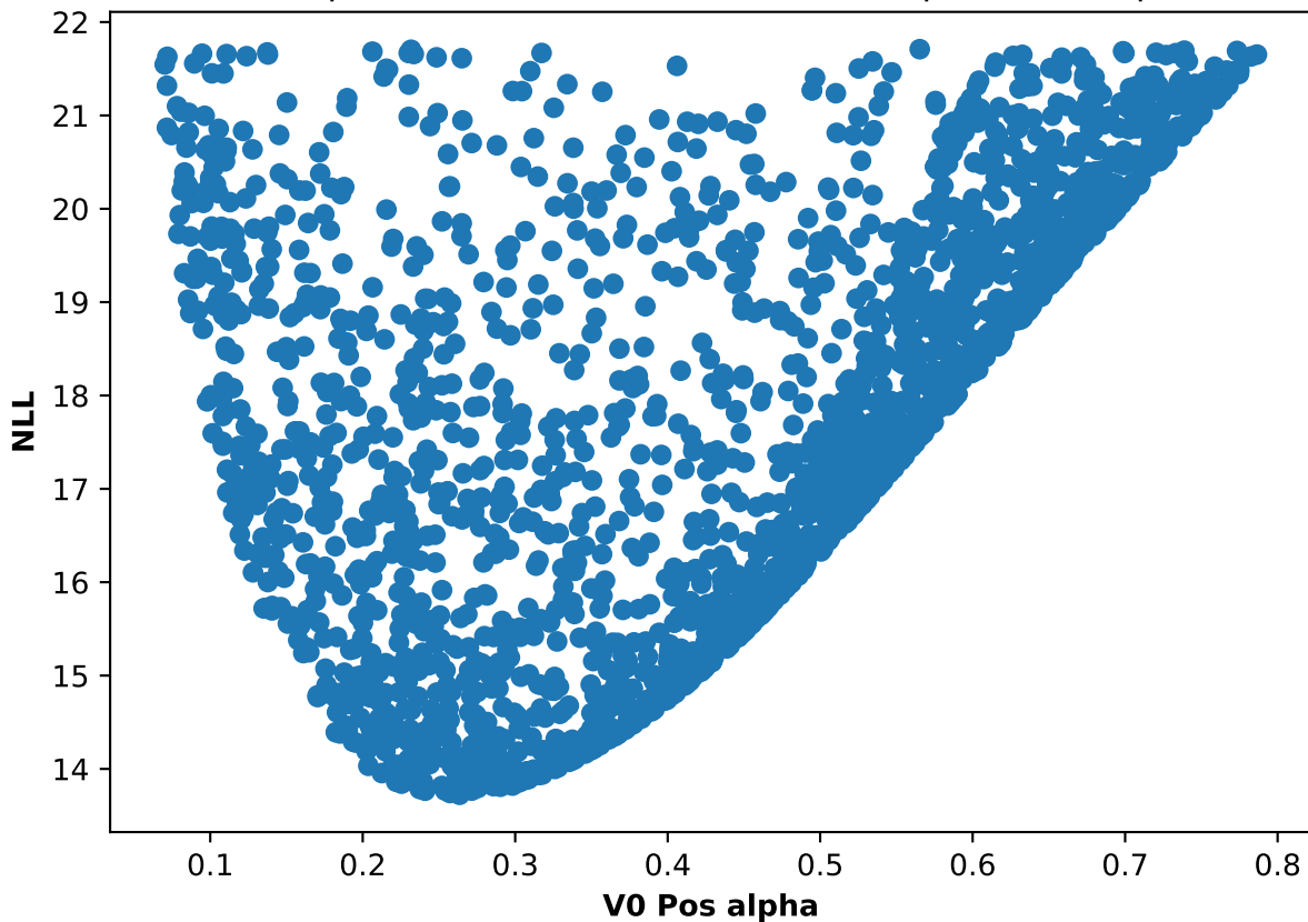
Participant 42, run 5: NLL and V0 Pos alpha scatter plot
