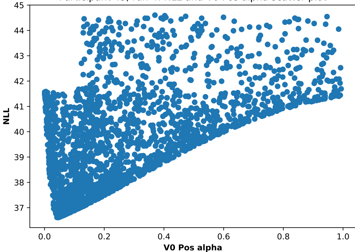
Participant 43, run 4: NLL and V0 Pos alpha scatter plot
