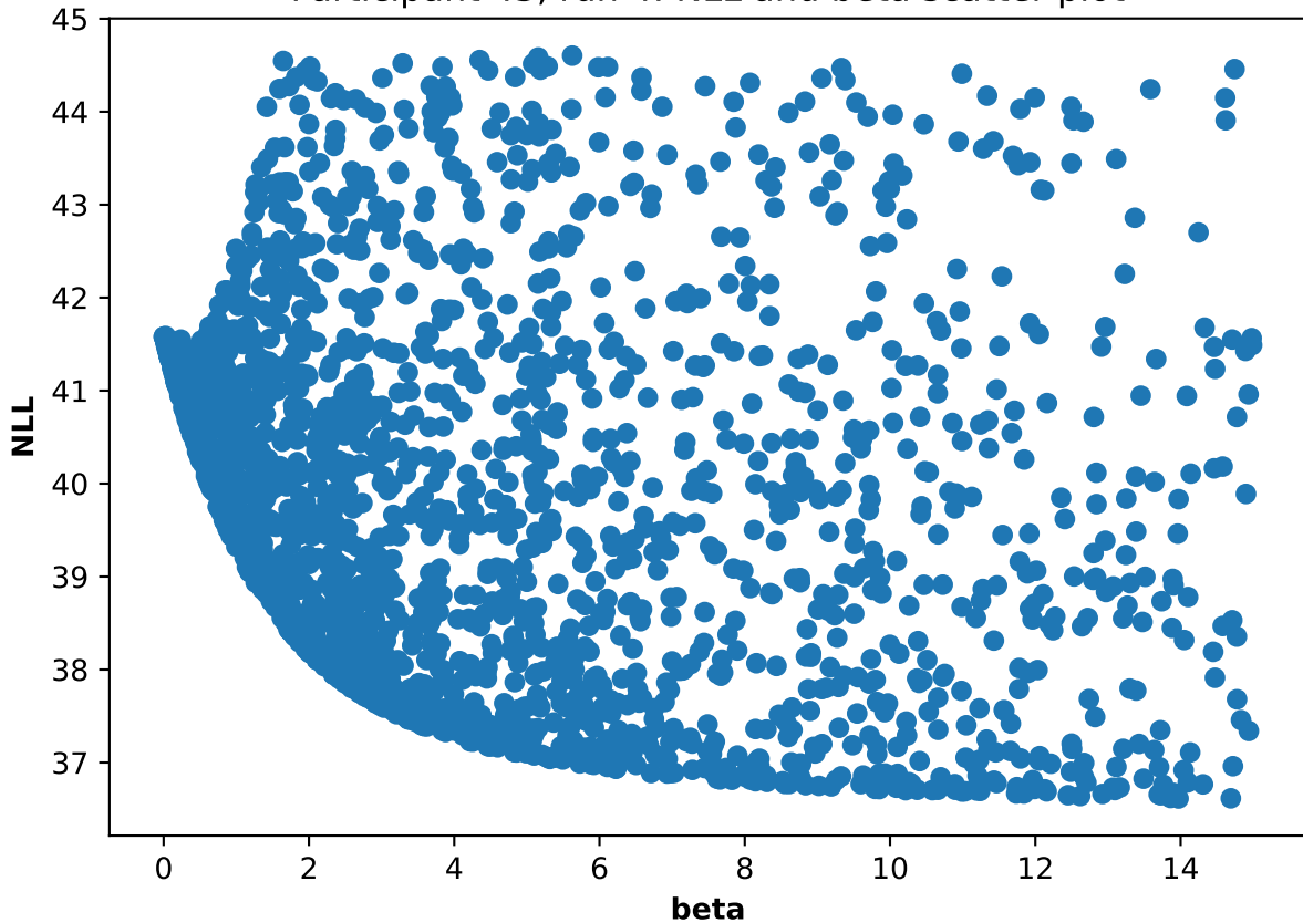
Participant 43, run 4: NLL and beta scatter plot
