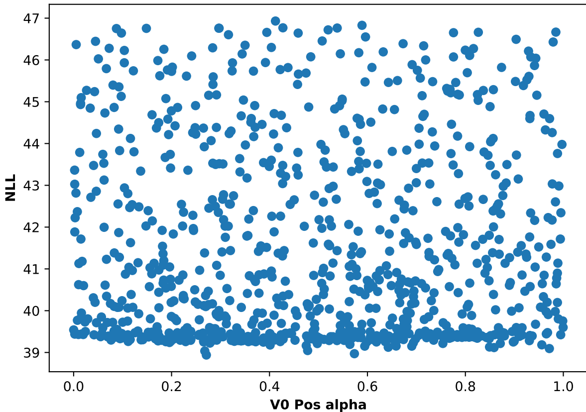
Participant 45, run 1: NLL and V0 Pos alpha scatter plot
