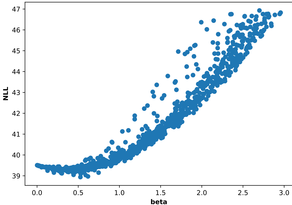
Participant 45, run 1: NLL and beta scatter plot
