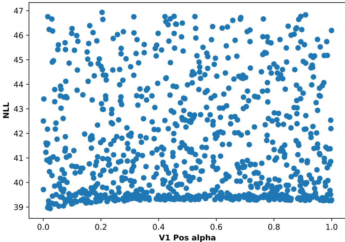
Participant 45, run 1: NLL and V1 Pos alpha scatter plot
