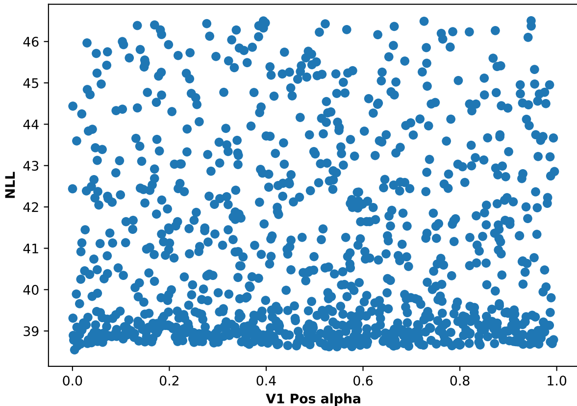
Participant 45, run 2: NLL and V1 Pos alpha scatter plot
