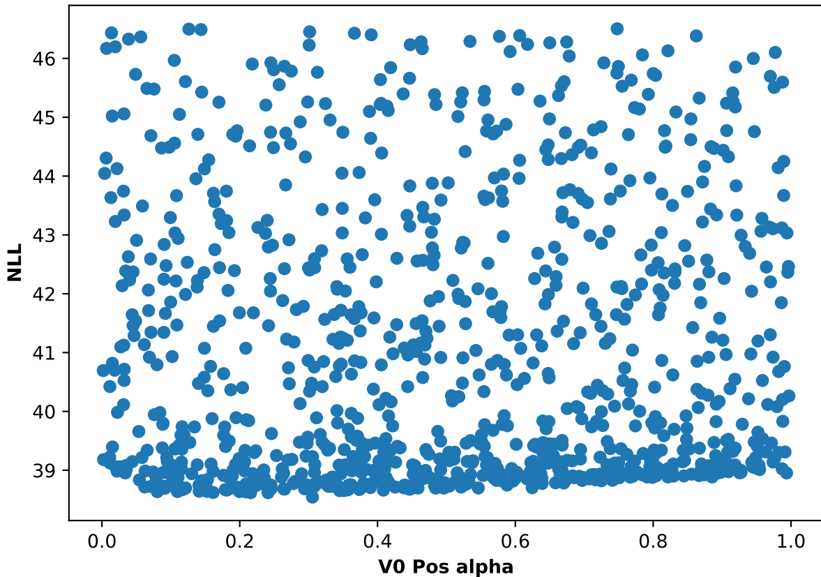
Participant 45, run 2: NLL and V0 Pos alpha scatter plot
