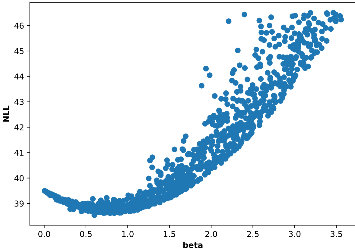
Participant 45, run 2: NLL and beta scatter plot
