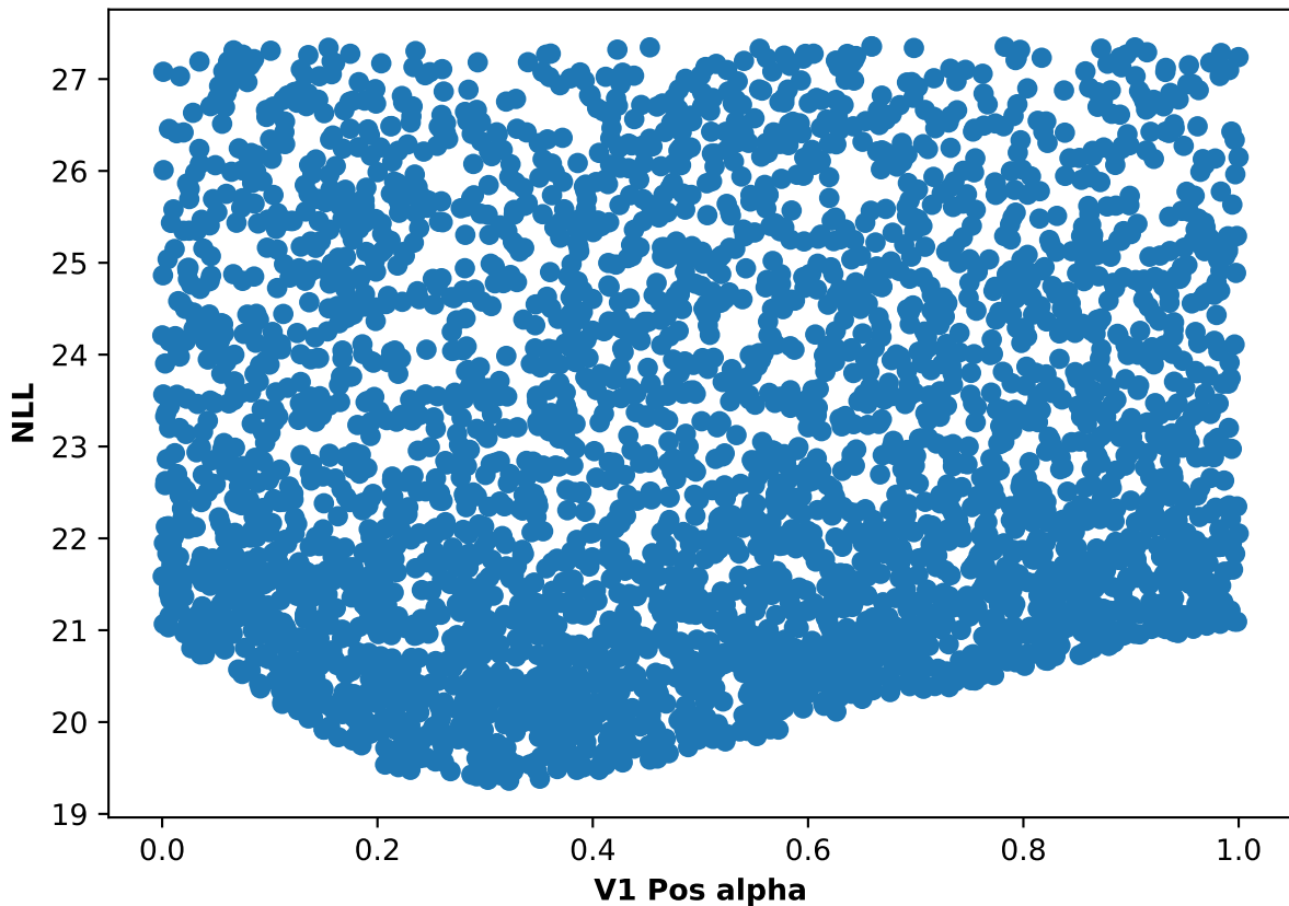
Participant 45, run 4: NLL and V1 Pos alpha scatter plot
