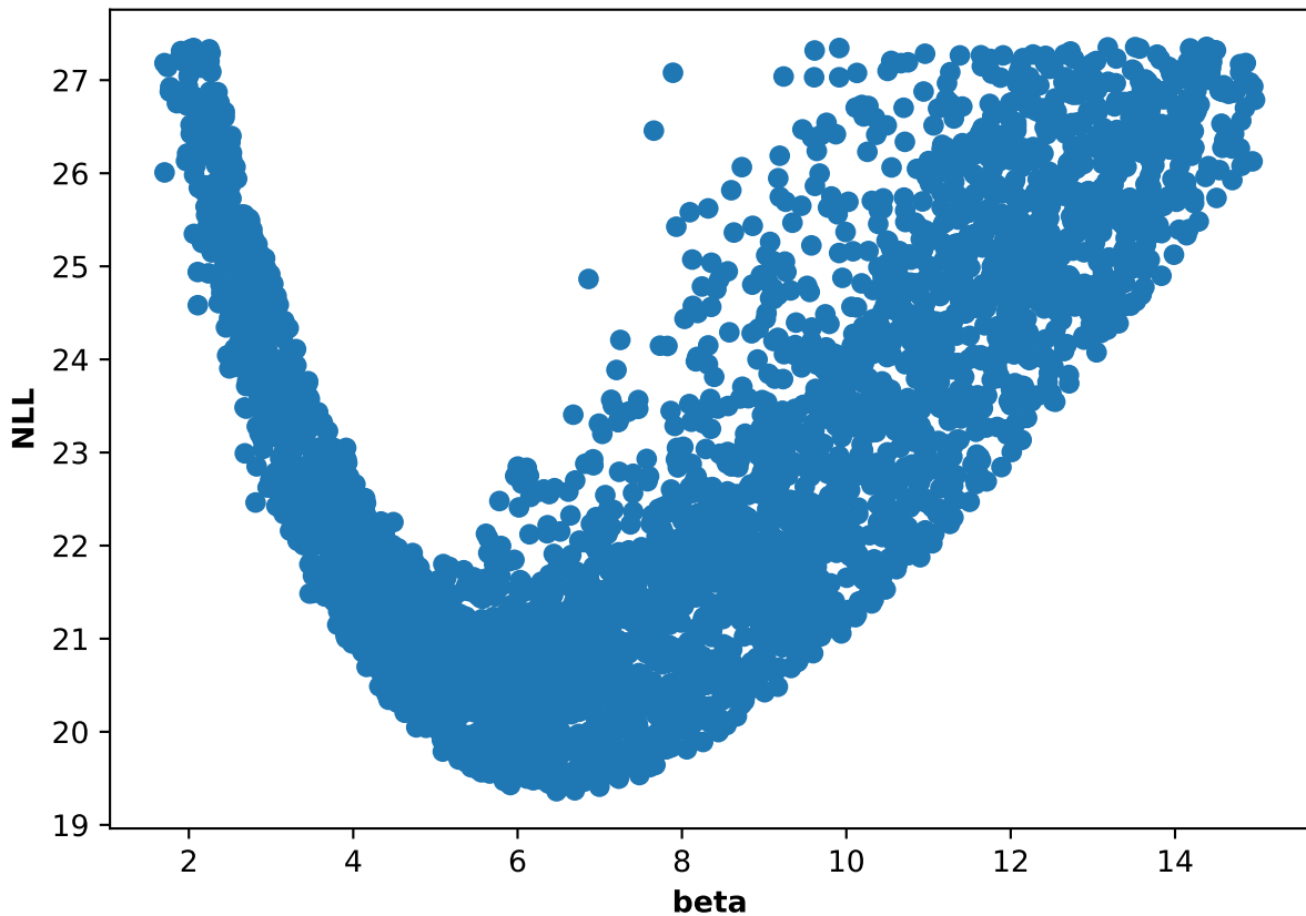
Participant 45, run 4: NLL and beta scatter plot
