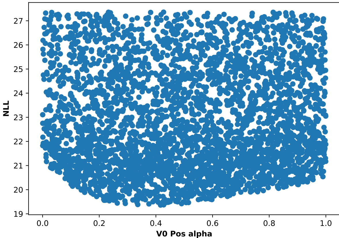
Participant 45, run 4: NLL and V0 Pos alpha scatter plot
