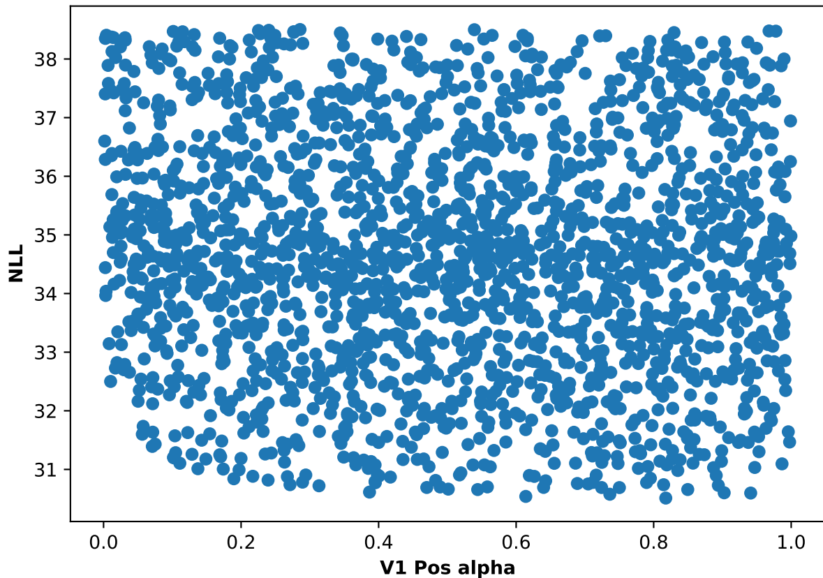
Participant 45, run 5: NLL and V1 Pos alpha scatter plot
