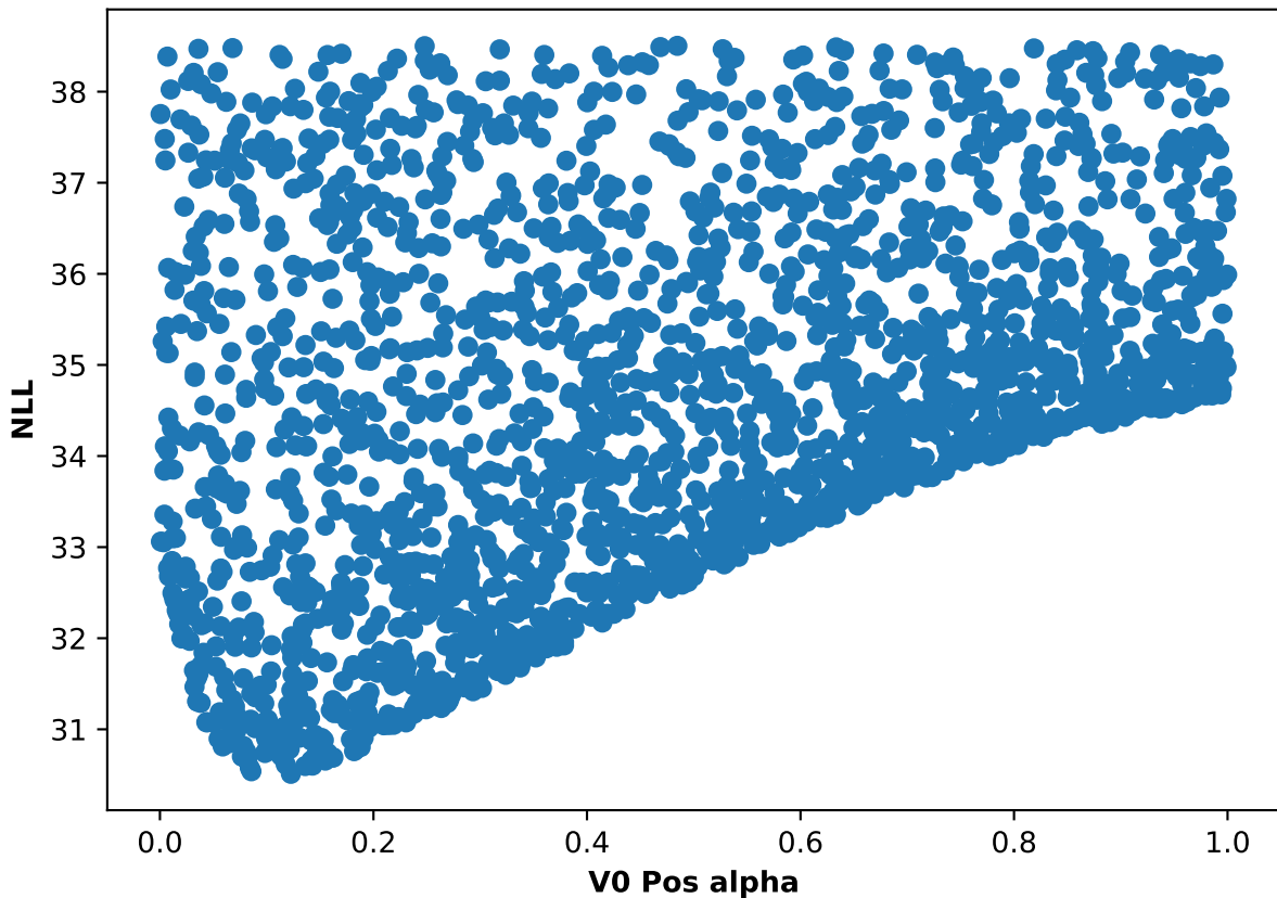
Participant 45, run 5: NLL and V0 Pos alpha scatter plot
