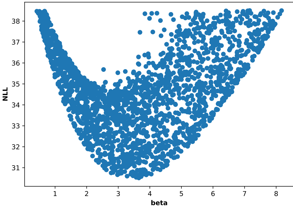
Participant 45, run 5: NLL and beta scatter plot
