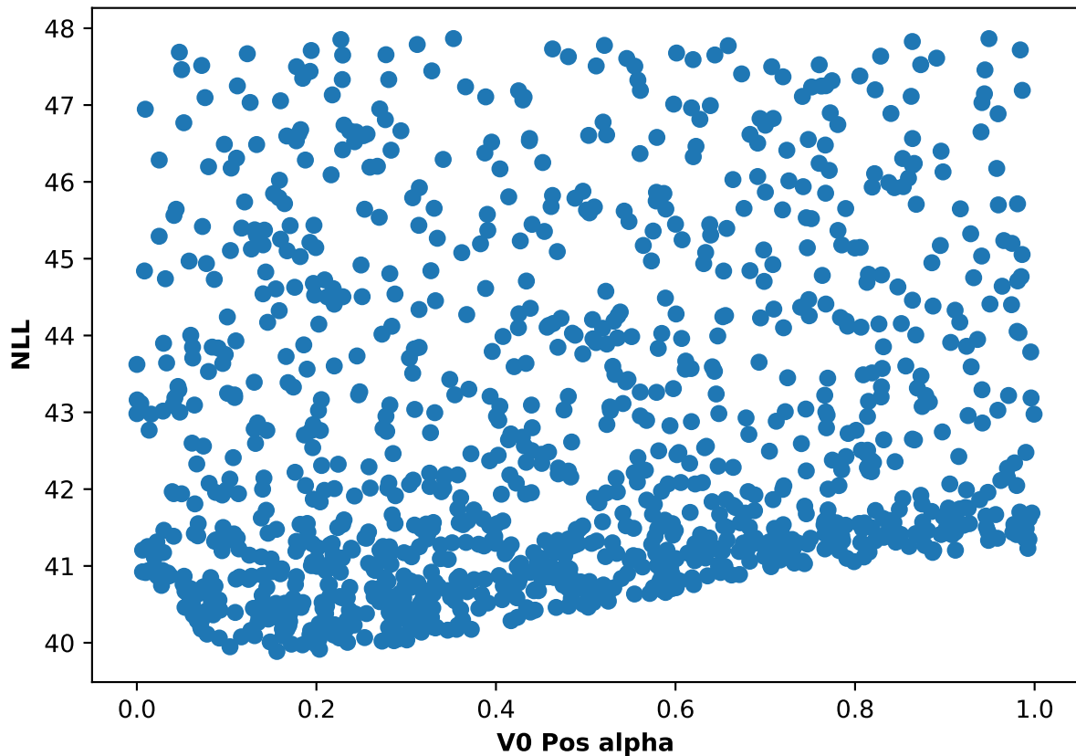
Participant 46, run 4: NLL and V0 Pos alpha scatter plot
