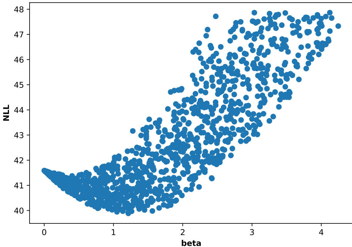
Participant 46, run 4: NLL and beta scatter plot
