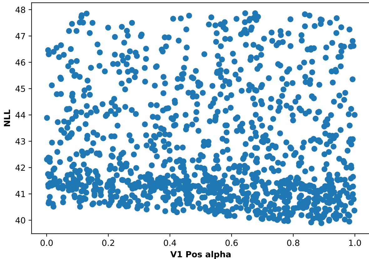
Participant 46, run 4: NLL and V1 Pos alpha scatter plot
