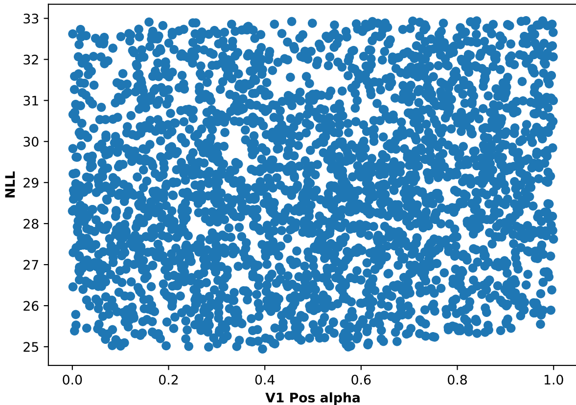
Participant 46, run 5: NLL and V1 Pos alpha scatter plot
