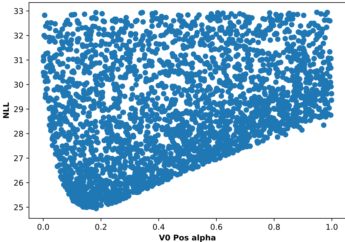
Participant 46, run 5: NLL and V0 Pos alpha scatter plot
