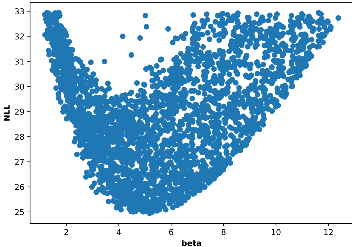
Participant 46, run 5: NLL and beta scatter plot
