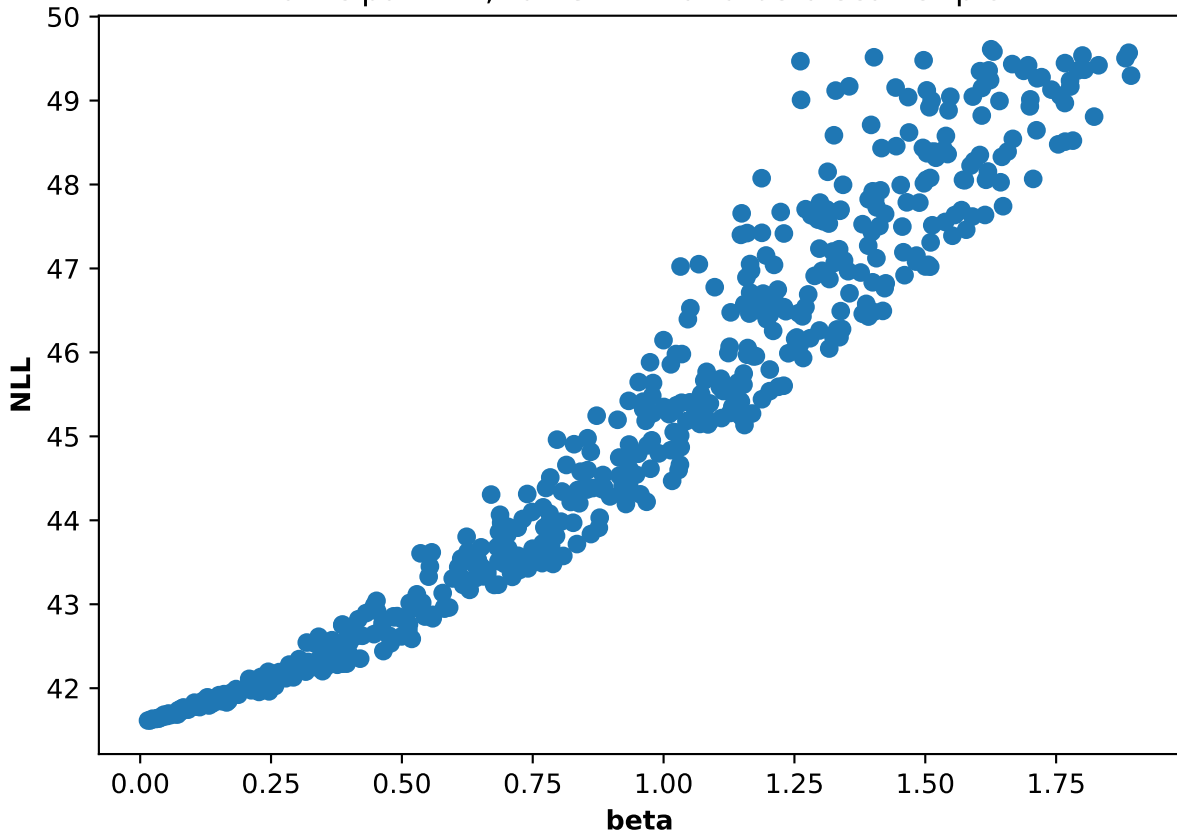
Participant 47, run 3: NLL and beta scatter plot
