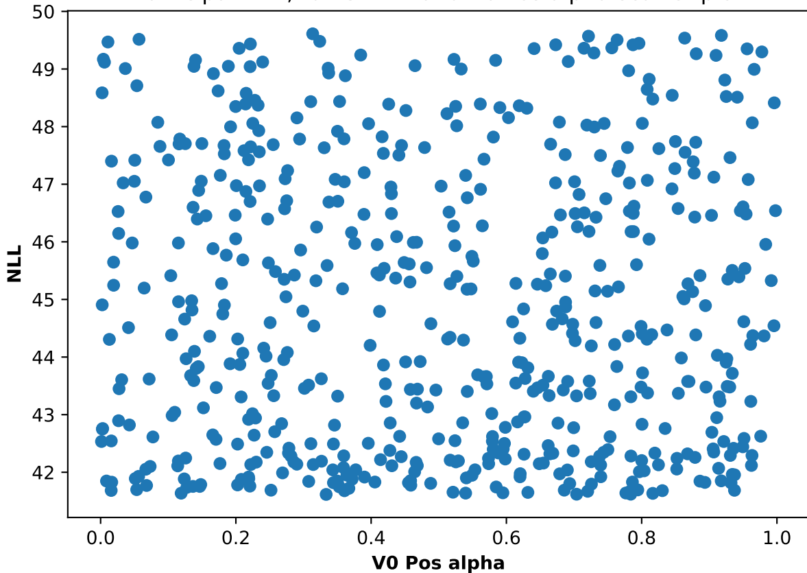
Participant 47, run 3: NLL and V0 Pos alpha scatter plot
