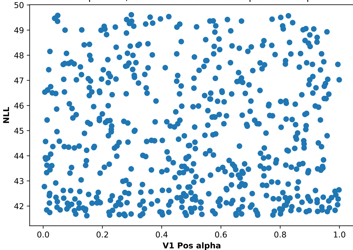
Participant 47, run 3: NLL and V1 Pos alpha scatter plot
