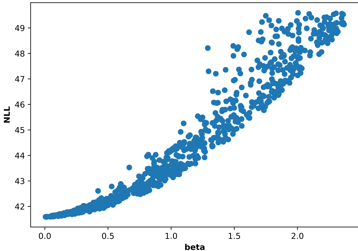
Participant 49, run 1: NLL and beta scatter plot
