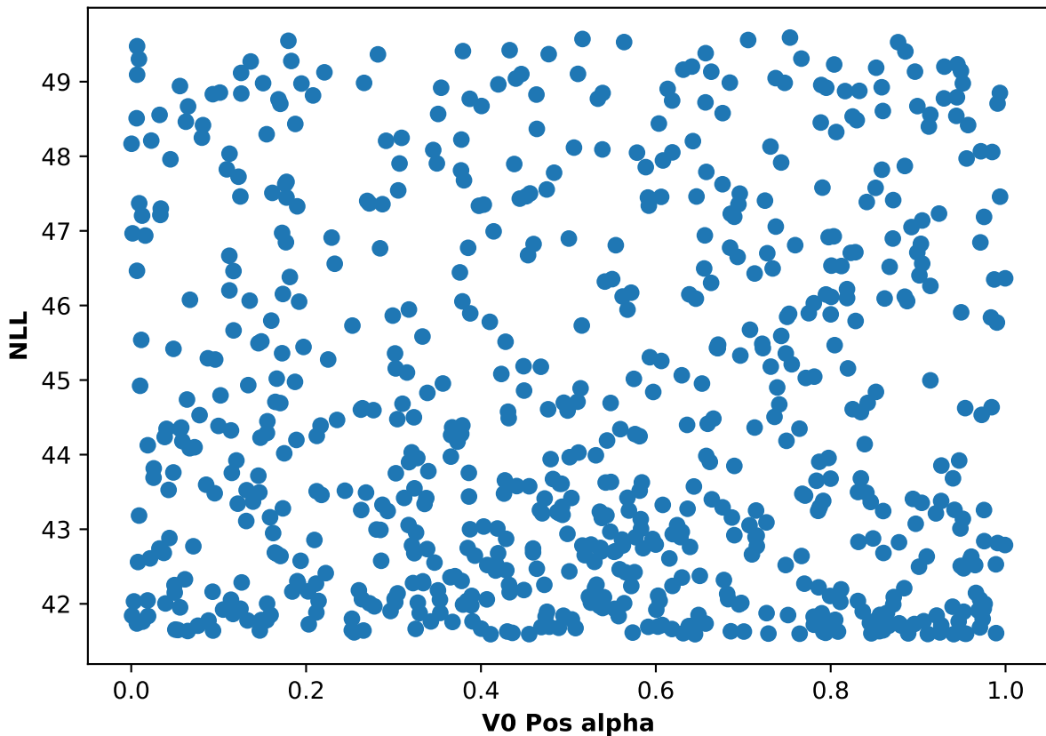
Participant 49, run 1: NLL and V0 Pos alpha scatter plot
