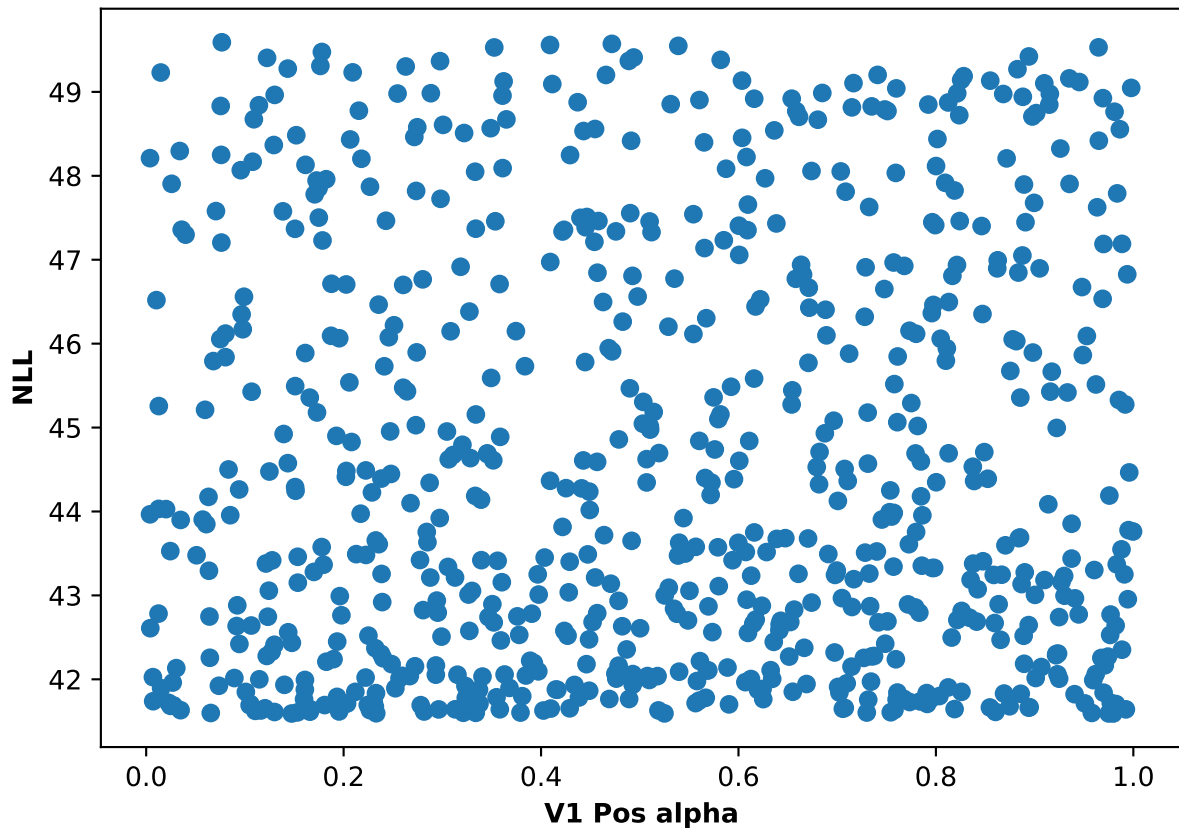
Participant 49, run 1: NLL and V1 Pos alpha scatter plot
