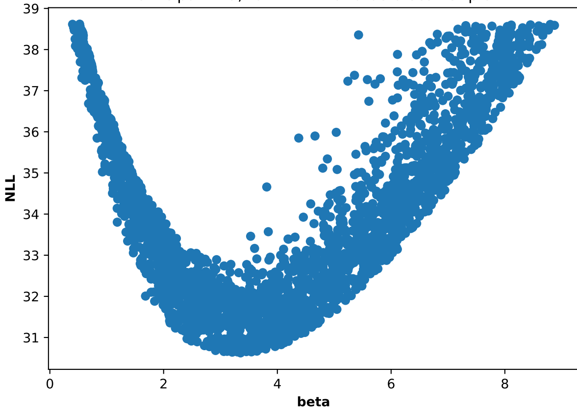
Participant 49, run 4: NLL and beta scatter plot
