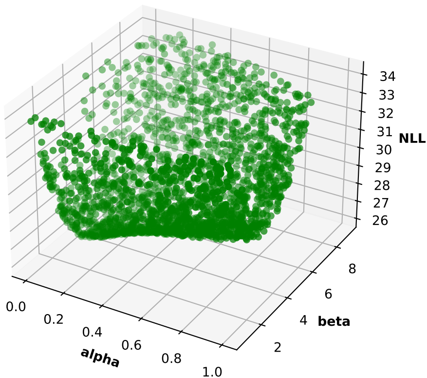
Participant 50, run 5: NLL, alpha and beta 3D scatter plot
