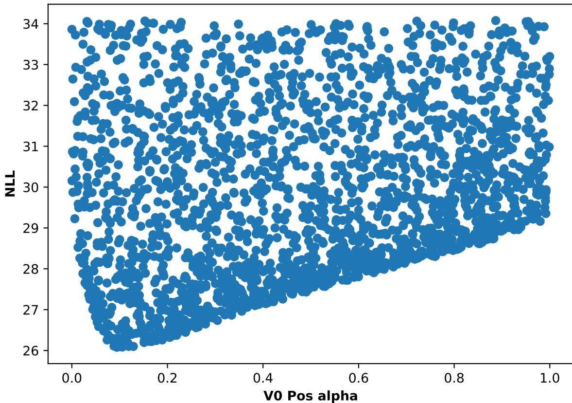
Participant 50, run 5: NLL and V0 Pos alpha scatter plot
