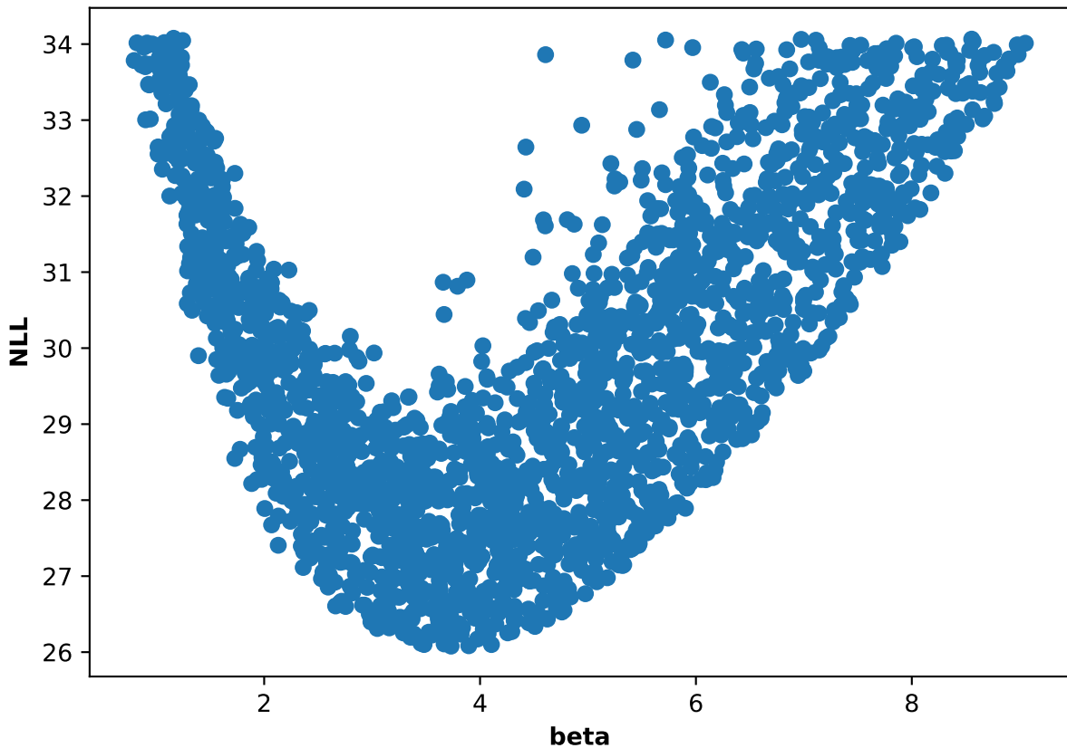
Participant 50, run 5: NLL and beta scatter plot
