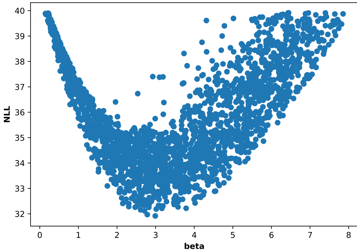
Participant 51, run 3: NLL and beta scatter plot
