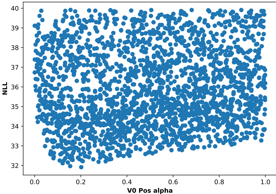
Participant 51, run 3: NLL and V0 Pos alpha scatter plot
