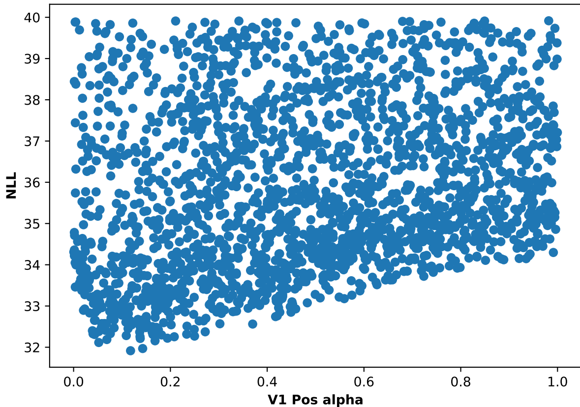
Participant 51, run 3: NLL and V1 Pos alpha scatter plot
