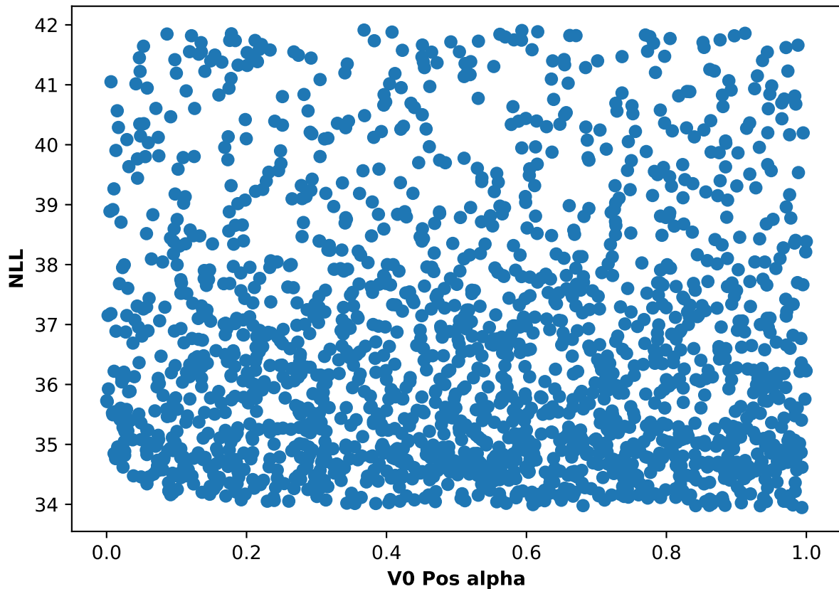
Participant 51, run 4: NLL and V0 Pos alpha scatter plot
