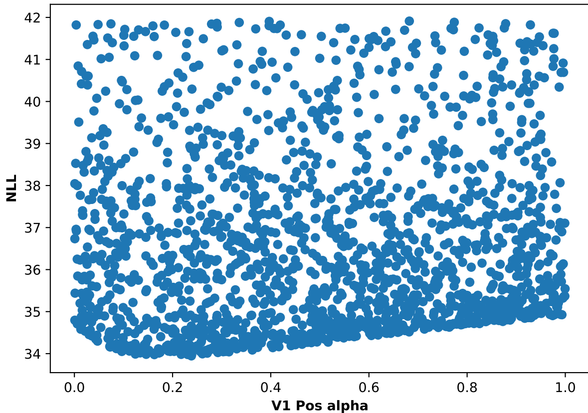
Participant 51, run 4: NLL and V1 Pos alpha scatter plot
