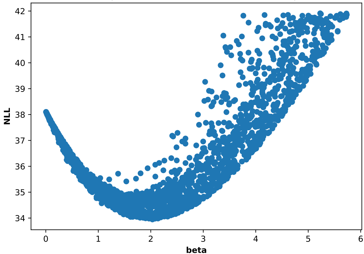
Participant 51, run 4: NLL and beta scatter plot
