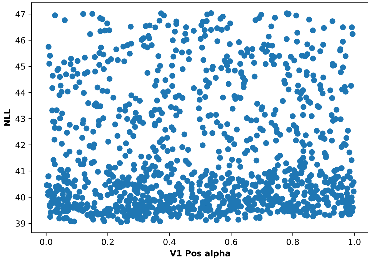
Participant 52, run 1: NLL and V1 Pos alpha scatter plot
