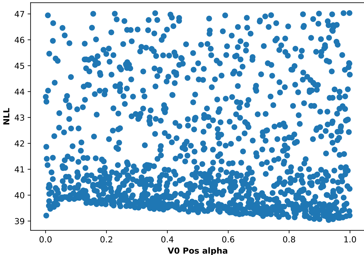
Participant 52, run 1: NLL and V0 Pos alpha scatter plot
