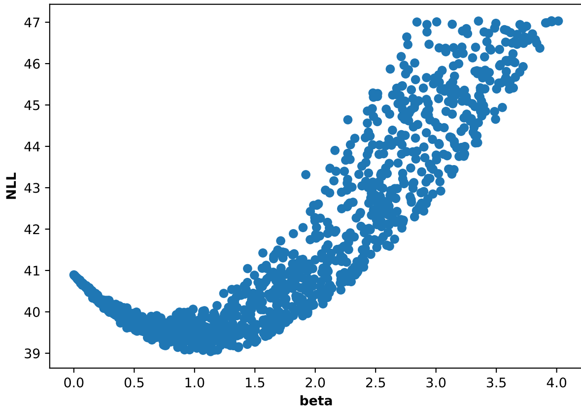
Participant 52, run 1: NLL and beta scatter plot
