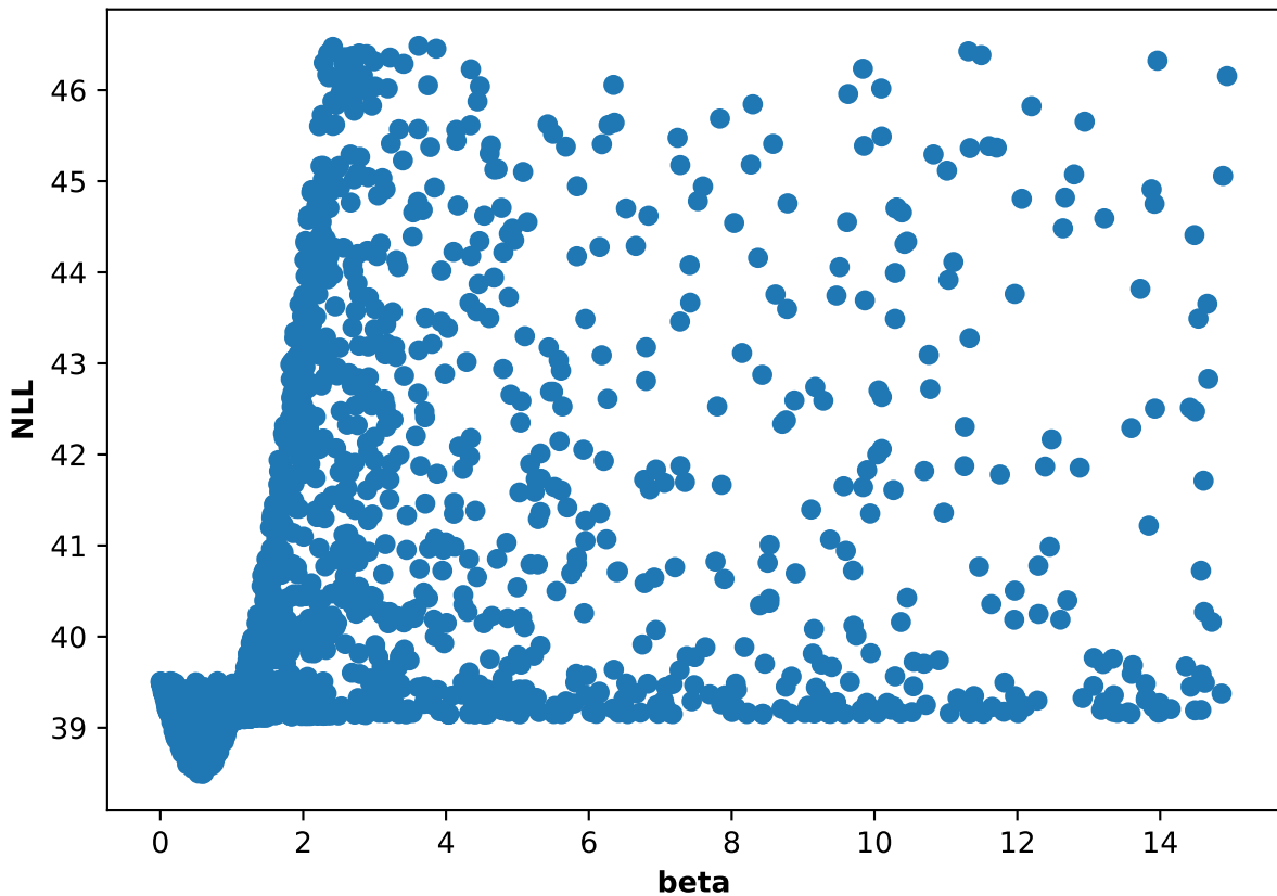
Participant 53, run 4: NLL and beta scatter plot
