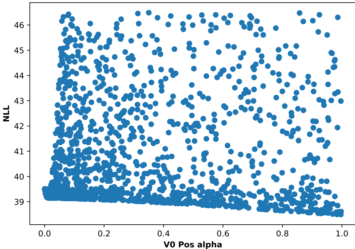
Participant 53, run 4: NLL and V0 Pos alpha scatter plot
