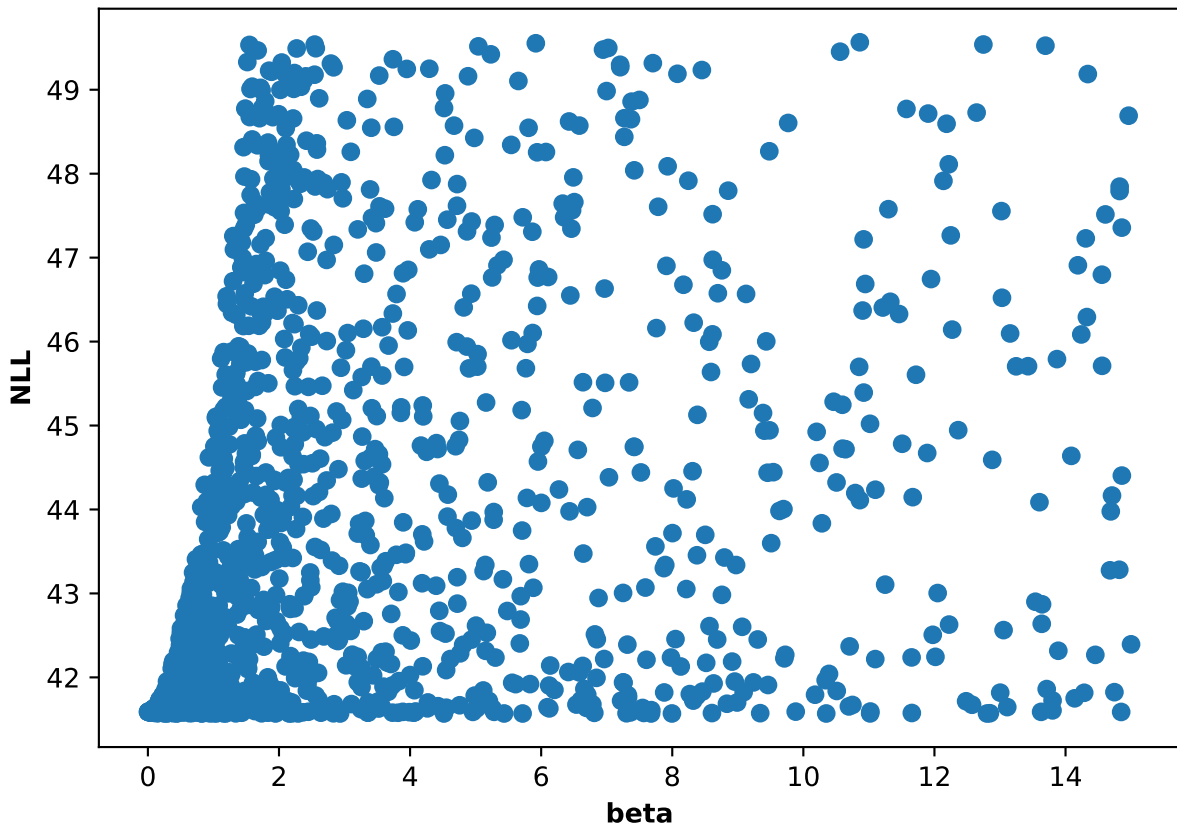
Participant 53, run 5: NLL and beta scatter plot
