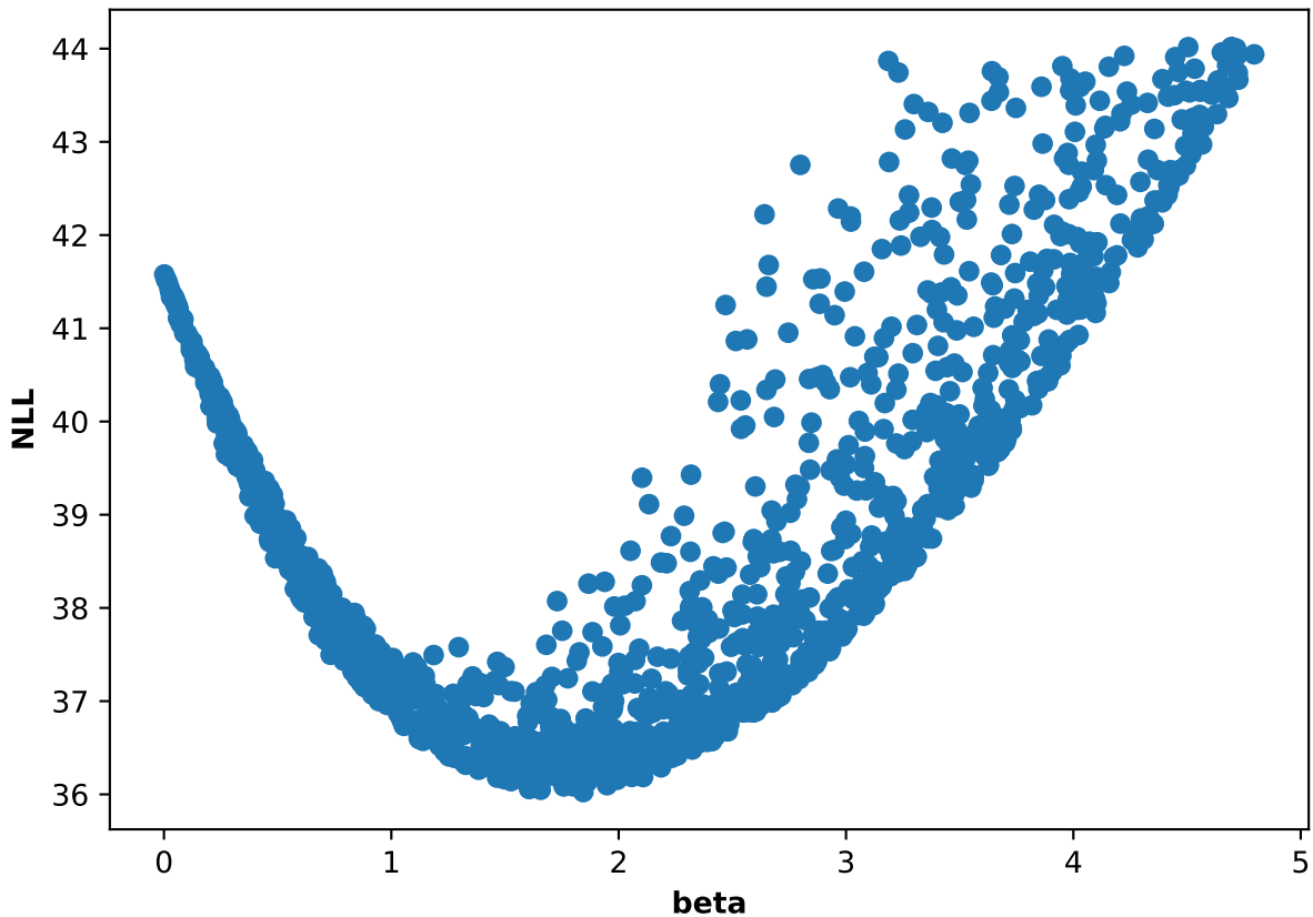
Participant 54, run 3: NLL and beta scatter plot
