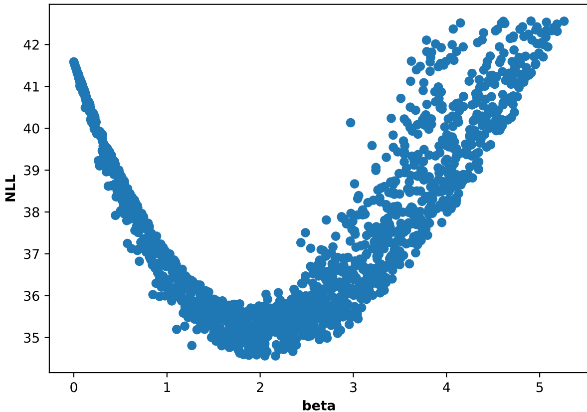
Participant 54, run 4: NLL and beta scatter plot
