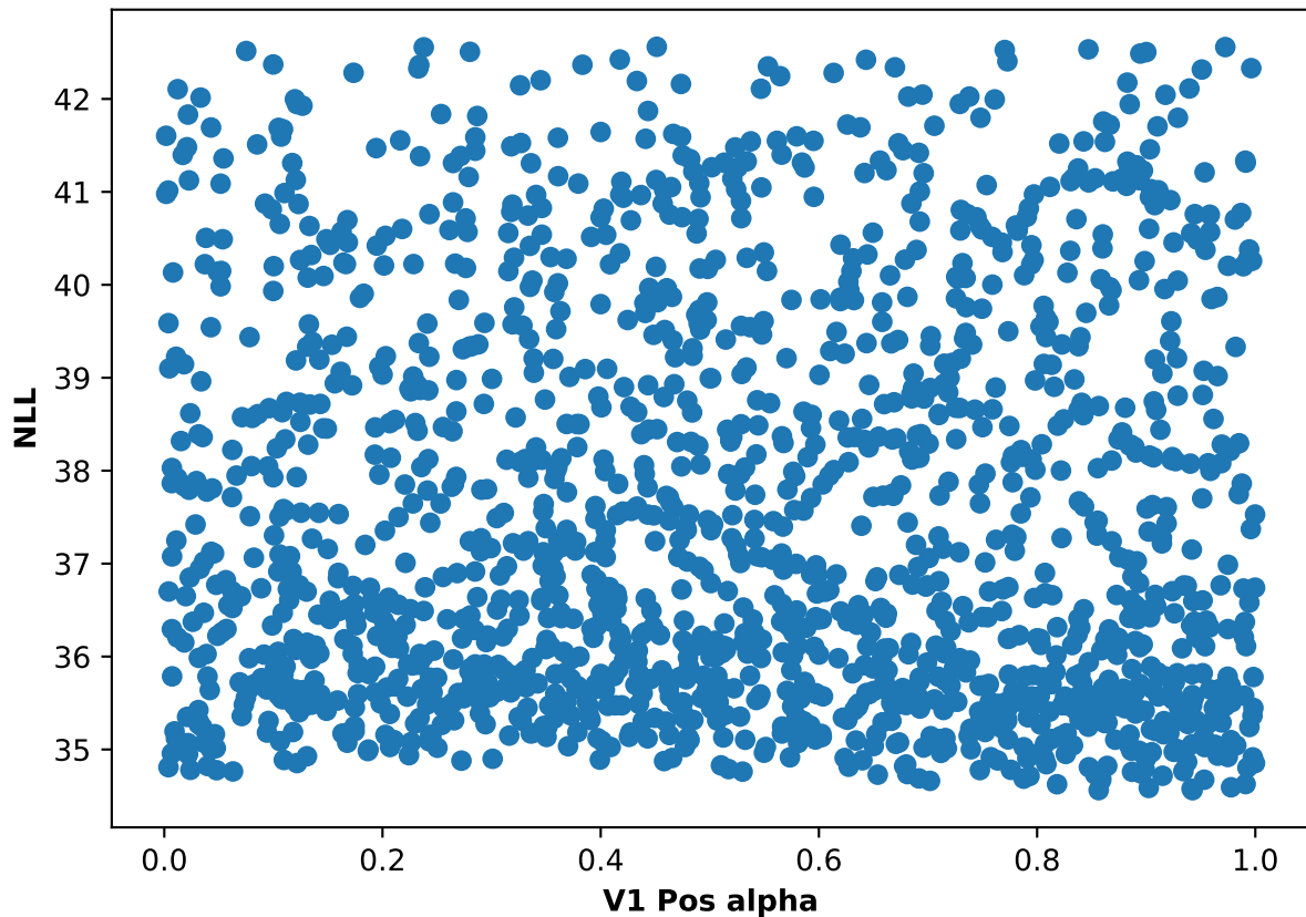
Participant 54, run 4: NLL and V1 Pos alpha scatter plot
