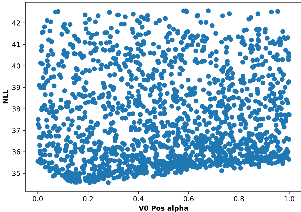
Participant 54, run 4: NLL and V0 Pos alpha scatter plot
