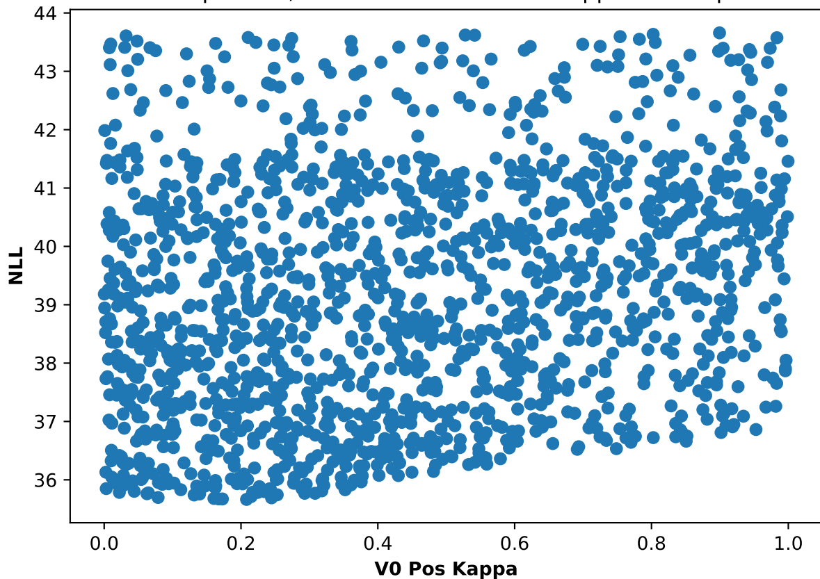
Participant 55, run 1: NLL and V0 Pos Kappa scatter plot
