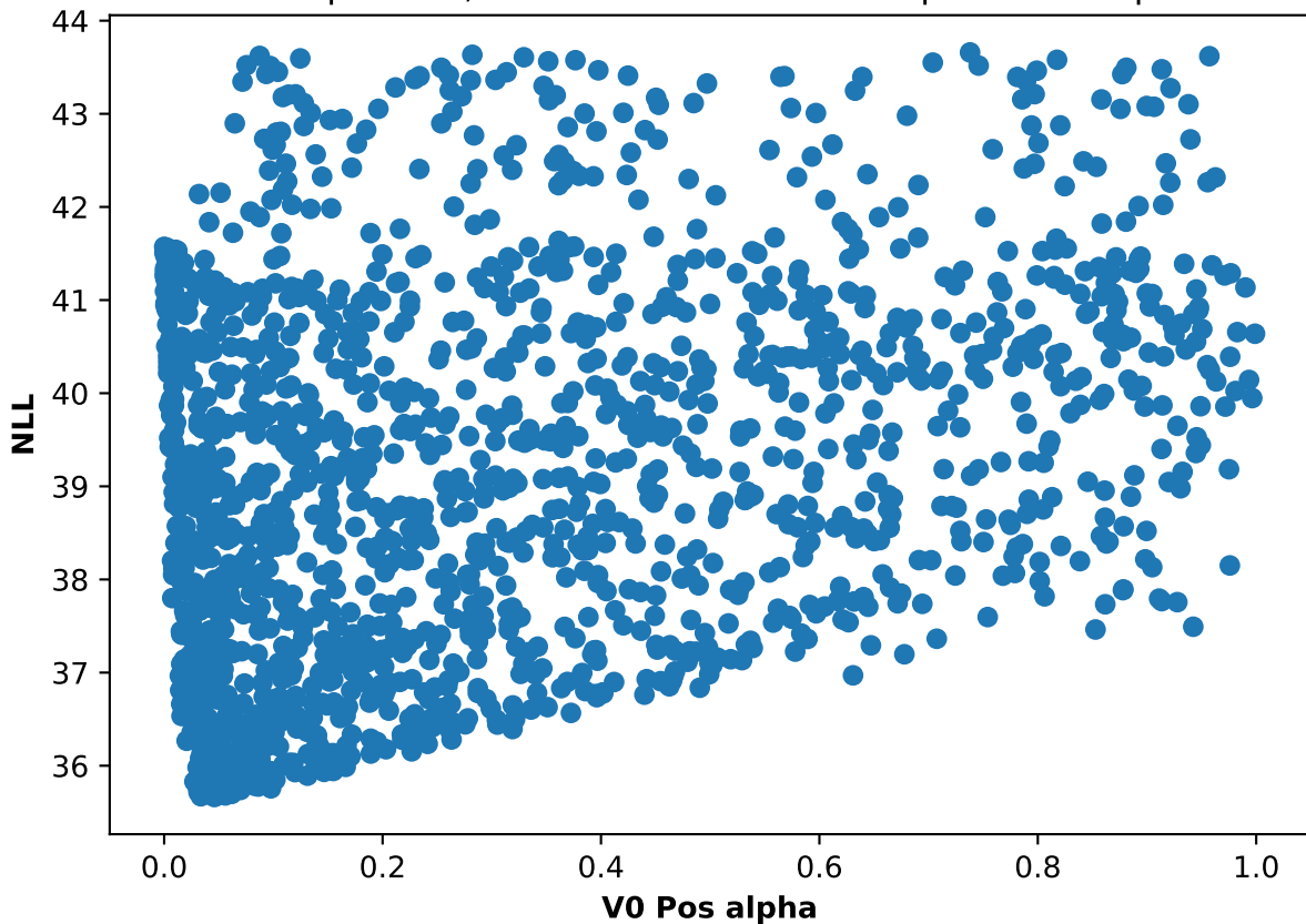
Participant 55, run 1: NLL and V0 Pos alpha scatter plot
