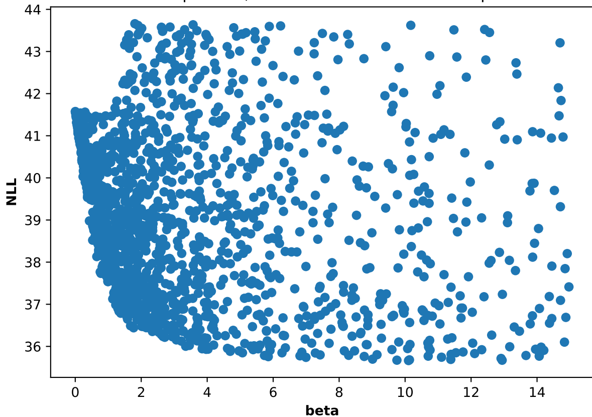
Participant 55, run 1: NLL and beta scatter plot
