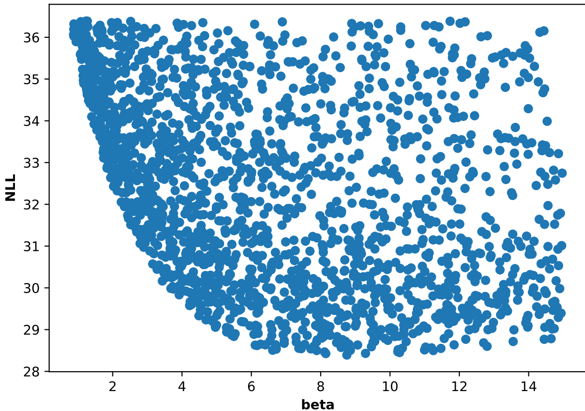
Participant 55, run 3: NLL and beta scatter plot
