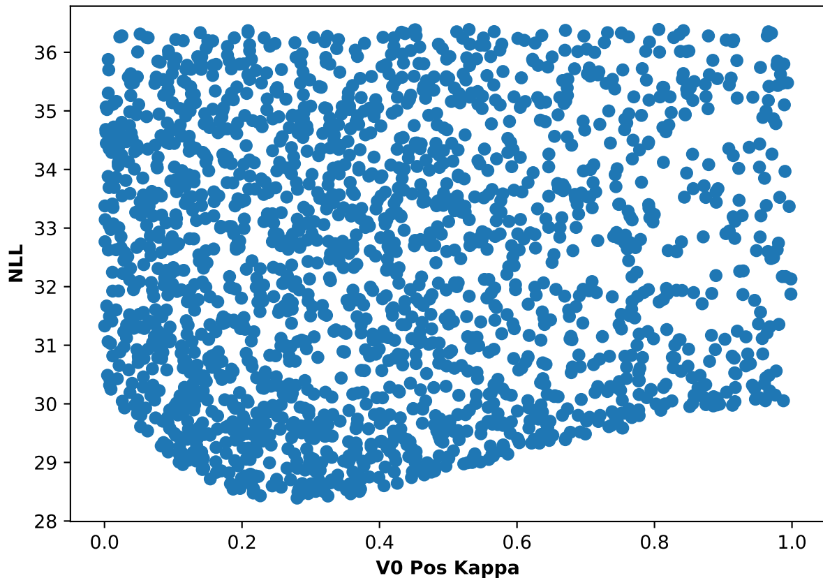
Participant 55, run 3: NLL and V0 Pos Kappa scatter plot
