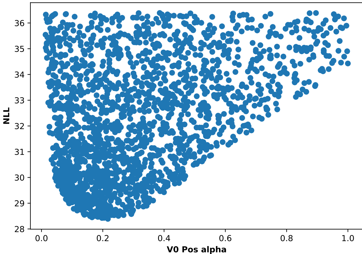
Participant 55, run 3: NLL and V0 Pos alpha scatter plot
