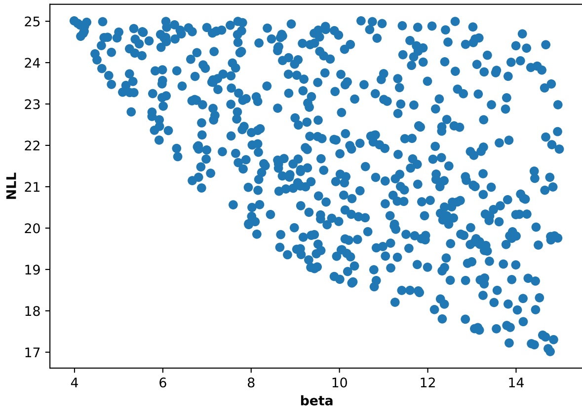
Participant 55, run 4: NLL and beta scatter plot
