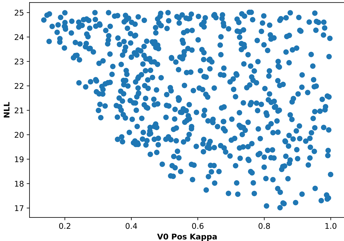
Participant 55, run 4: NLL and V0 Pos Kappa scatter plot
