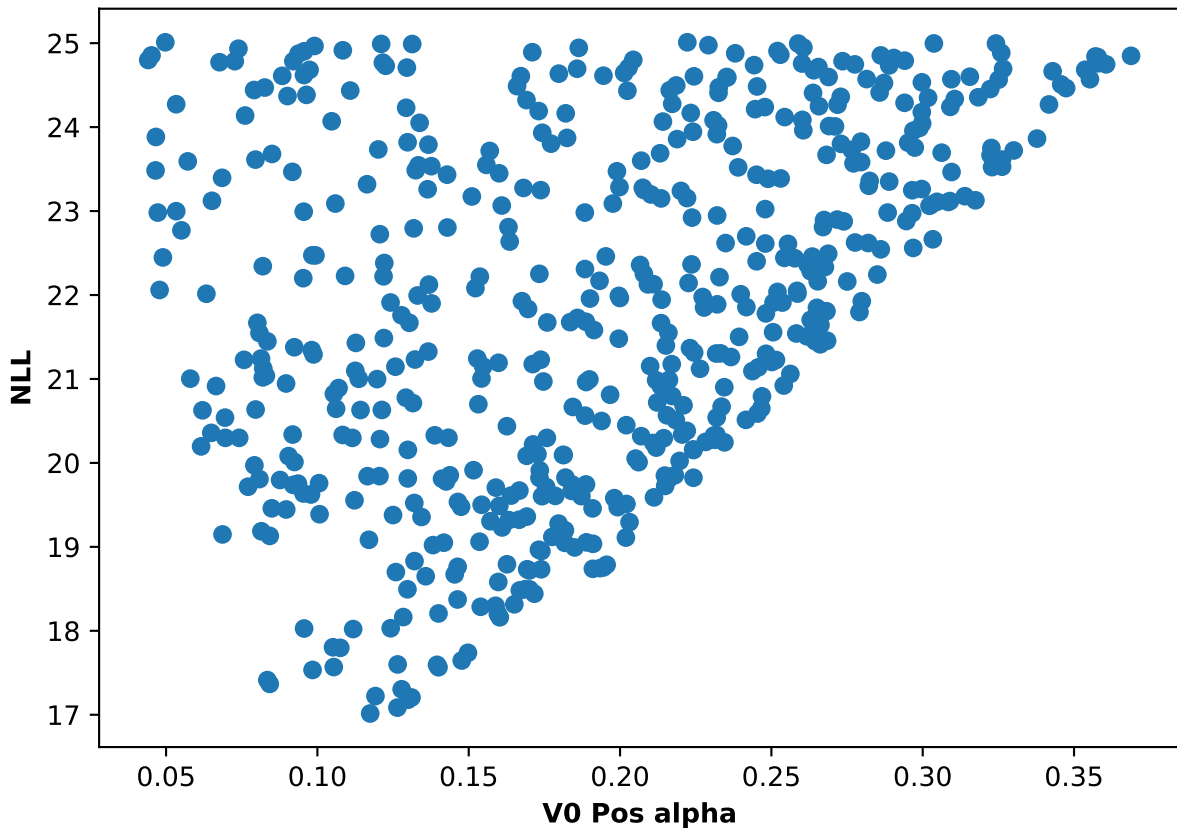
Participant 55, run 4: NLL and V0 Pos alpha scatter plot
